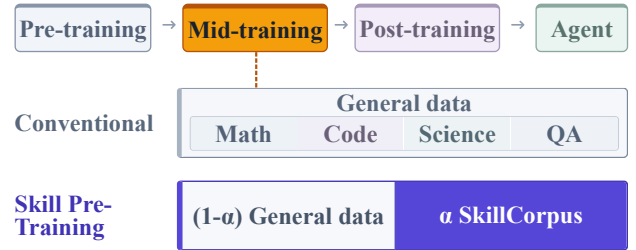
(b) SPT as mid-training composition.
