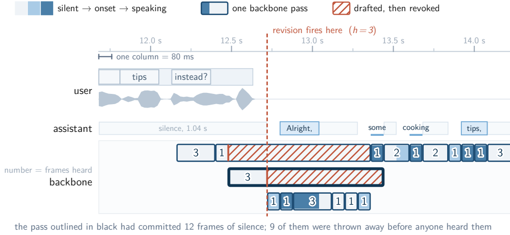
Figure 9: Revision after partial draft consumption. For DiffuPlex-SPEAK, the highlighted backbone pass drafts 12 frames of assistant silence. Revision fires after three frames have been consumed, discarding the remaining nine unplayed frames before a new assistant continuation is generated. Hatched regions denote drafted frames that are revoked before playback.
