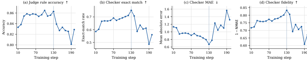
Figure 8: HealthBench diagnostics on the Qwen3.5-9B trajectory. Same four panels as Figure 7, now on the different-style medical suite that PAV never sees. (a) Judge rule accuracy (↑). (b) Checker exact-match rate (↑). (c) Checker MAE on the 0–4 scale (↓); malformed checker outputs receive their worst possible endpoint error. (d) Checker fidelity 1 - \text{NMAE} = 1 - \text{MAE}/4 (↑). Dotted lines and enlarged markers mark the PAV landmark @130. Judge accuracy, exact match, and fidelity peak together around that region and then fall together, so the transfer suite tracks the same useful window as the SV-HARD monitor.
