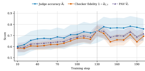
Figure 4: PAV on SV-HARD (RQ3) . Judge accuracy \hat{A}_t , checker fidelity 1 - \hat{e}_{C,t} , and composite \hat{V}_t (dashed; 95% CI). Dotted line denotes the PAV landmark (step 130).
