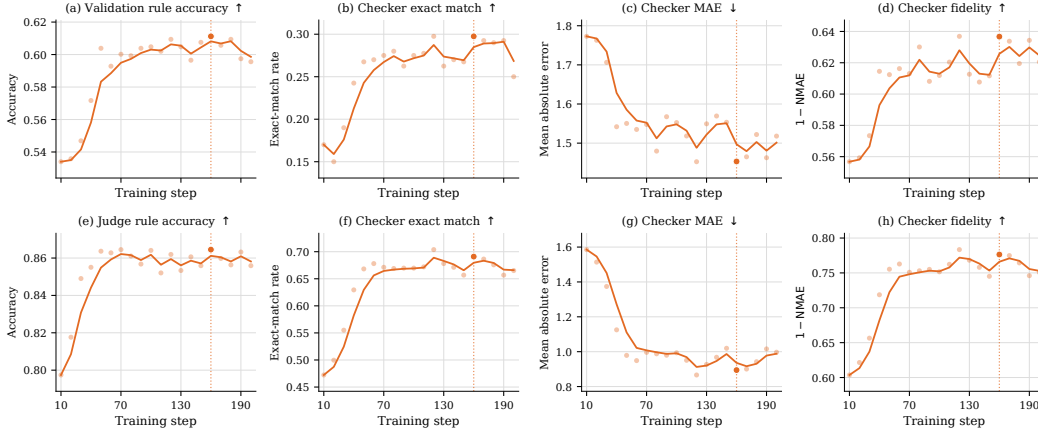
Figure 9: Gemma judge and checker dynamics (RQ3 replication). Top row: SV-HARD diagnostics; bottom row: HealthBench diagnostics on the Gemma-4-E4B-it trajectory (steps 10–200). Same four panels as Figures 7 and 8. Dotted lines and enlarged markers mark the PAV landmark @160. Rule accuracy alone can continue to rise on SV-HARD, whereas exact match, MAE, and fidelity expose the checker-quality window that motivates stopping.
