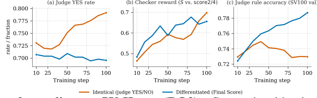
Figure 3: Interface decoupling on SV-HARD (RQ2). Comparing identical YES/NO checking against differentiated Final Score (steps 10–100). (a) Identical checking inflates YES rate. (b) Both report climbing rewards ( [0, 1] scale). (c) Only the differentiated Final Score converts reward growth into genuine validation accuracy gains.
