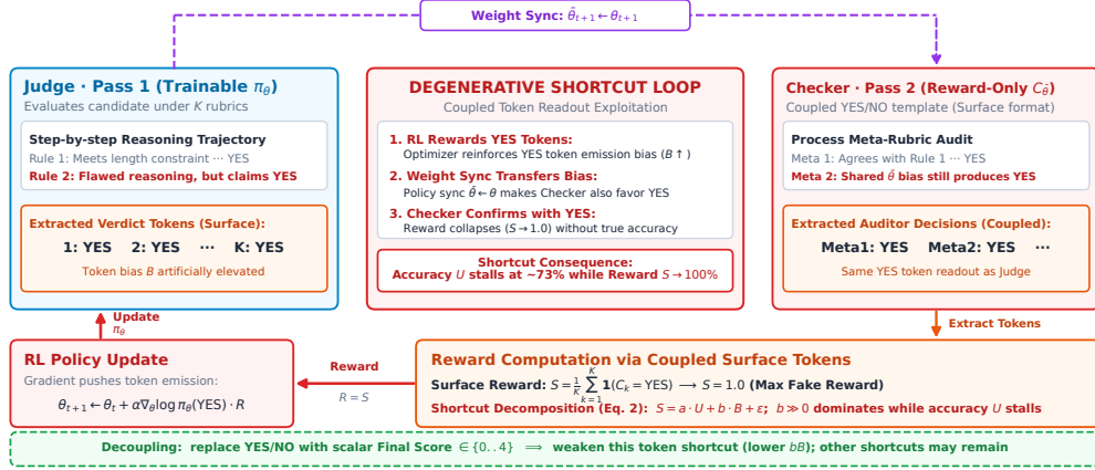
Figure 5: Surface coupling and the degenerative reward shortcut pathway (Section 3.2). When Judge (Pass 1) and Checker (Pass 2) share identical YES/NO readout templates, self-produced reward S is extracted directly from surface decision tokens ( S = \frac{1}{K} \sum \mathbf{1}(\text{Checker}_k = \text{YES}) ). Policy gradient optimization inflates YES token emission ( B \uparrow ), transferring immediately to synchronized checker weights ( \hat{\theta} \leftarrow \theta ). This establishes a degenerative shortcut loop ( bB ) where self-assigned rewards surge to 100% while true evaluative capability U stalls. Interface decoupling replaces the checker’s verdict surface with a free-standing 5-tier scalar Final Score, severing this direct token-level shortcut channel.
