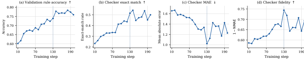
Figure 7: SV-HARD diagnostics on the Qwen3.5-9B trajectory. (a) Validation rule accuracy ( \uparrow ). (b) Checker exact-match rate ( \uparrow ). (c) Checker MAE on the original 0–4 score scale ( \downarrow ); malformed checker outputs receive their worst possible endpoint error. (d) Checker fidelity 1 - \text{NMAE} = 1 - \text{MAE}/4 ( \uparrow ). Dotted lines and enlarged markers show the PAV landmark @ 130. Rule accuracy alone continues to rise, whereas exact match, MAE, and fidelity expose the sharp checker improvement around the selected checkpoint.
