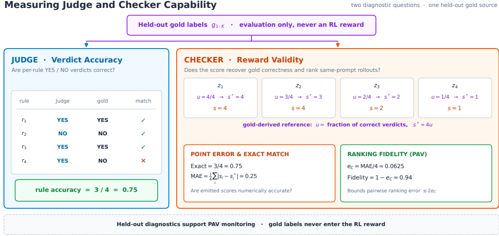
Figure 6: Gold-derived diagnostics for judge and checker capability on a four-rollout example. The same held-out rule labels simultaneously evaluate judge rule accuracy ( A ) and the checker reference target U = 4u (where u is gold rule correctness). Checker diagnostics evaluate point error (MAE and Exact match) and normalized ranking fidelity ( 1 - e_C = 1 - NMAE ), directly supplying the PAV composite monitor ( V ). Gold labels never enter the RL training reward.
