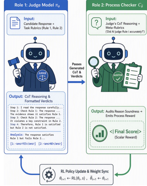
Figure 1: Overview of RECURSE. Trainable judge \pi_\theta evaluates responses under rubrics (Pass 1); synchronized checker C_{\bar{\theta}} audits reasoning against meta-rubrics to yield scalar process reward s (Pass 2). Policy parameters \theta are updated via RL on s , and checker weights \bar{\theta} are synchronized each step ( \bar{\theta}_{t+1} \leftarrow \theta_{t+1} ).
