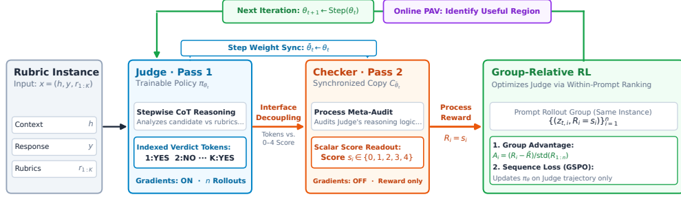
Figure 2: The RECURSE closed-loop optimization recurrence. Pass 1: trainable judge \pi_{\theta_t} emits reasoning and per-rule YES/NO verdicts on x = (h, y, r_{1:K}) ( n rollouts). Pass 2: a synchronized copy C_{\bar{\theta}_t} audits reasoning against meta-rubrics and returns a differentiated scalar score s_i \in \{0, \dots, 4\} as the sole reward. Interface decoupling closes direct token copying; the checker synchronizes parameters every step ( \bar{\theta}_t \leftarrow \theta_t ) without independent gradients. Online PAV monitoring on a human-verified validation set localizes early stopping.
