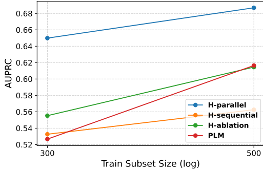
Figure 6: Comparison of models’ Dynamic mean AUPRC learning curves on GITHUB, plotted against training subset size.
