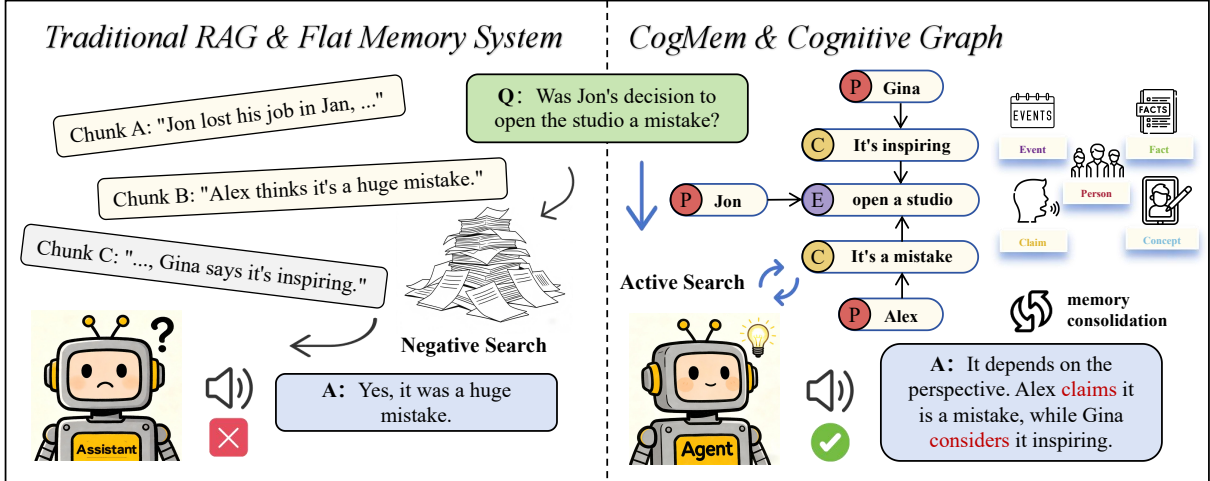
Figure 1: The Paradigm Shift from Passive Retrieval to Active Reconstruction. Left (traditional RAG and flat memory): passive retrieval over coarse text chunks introduces noise and may miss relevant counter-evidence. Even when a related statement is retrieved, the flat representation obscures its source and can cause the LLM to treat an attributed opinion as an unqualified record. Right (CogMem): a PEC 2 F cognitive graph supports active reconstruction, allowing the agent to attribute conflicting viewpoints to their sources and synthesize an evidence-grounded answer.
