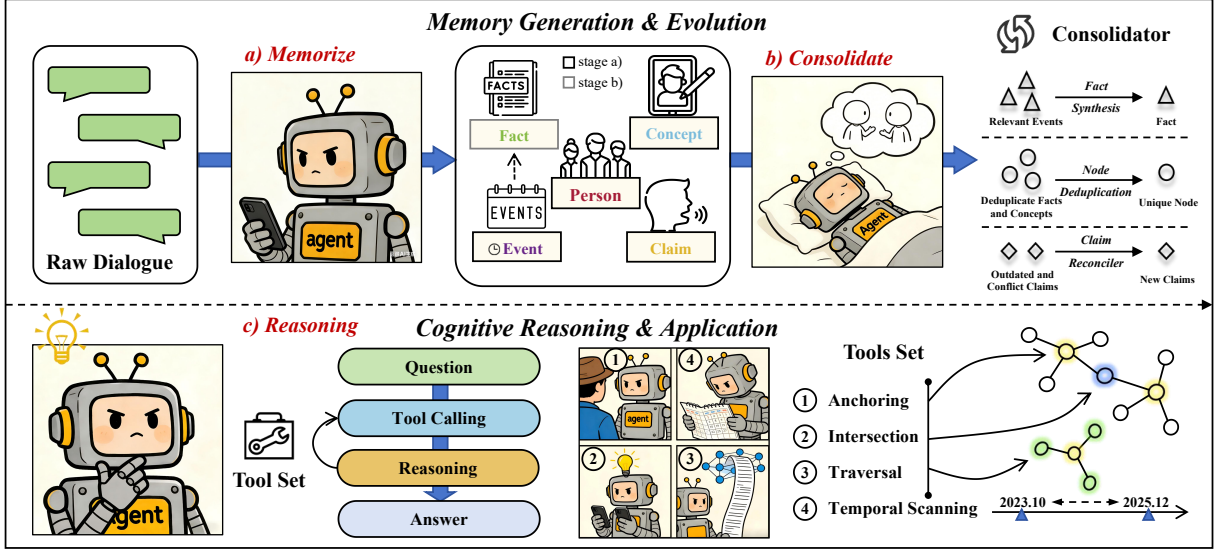
Figure 2: The Overall Architecture of CogMem. The framework consists of two layers: (1) Memory Generation & Evolution (Top) : (a) Memorize : The system processes raw dialogue to build an initial cognitive graph, converting episodic traces into graph nodes. (b) Consolidate : An offline mechanism synthesizes Facts from Events, merges duplicate Facts and Concepts, and reconciles temporally conflicting Claims into provenance-linked views without collapsing disagreements across speakers. (2) Cognitive Reasoning & Application (Bottom) : (c) Reasoning : Instead of passive retrieval, the Search Agent actively recalls information using a specialized Tool Set (Anchoring, Intersection, Traversal, Evidence Grounding) to dynamically navigate the graph and reconstruct answers through a ReAct loop.
