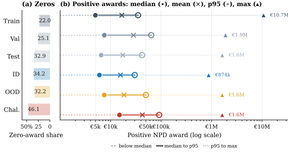
Figure 2: Award distribution across splits and diagnostic views. Panel (a) shows the zero-award share. Panel (b) shows the distribution of positive awards on a log scale, with markers for the median, mean, p95, and maximum.
