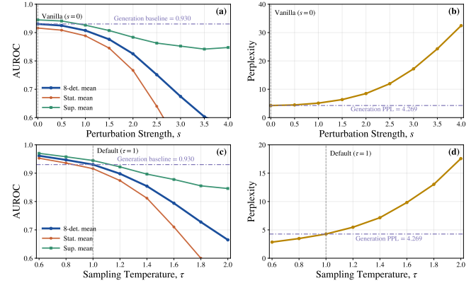
Fig. 1. Effects of decoding changes on AIGT detection and text quality. AUROC and perplexity under (a,b) top- k logit perturbation with strength s at \tau = 1 and (c,d) varying sampling temperature without logit perturbation. AUROC curves show means over all eight detectors and within two groups: statistical (Likelihood [1], Entropy and LogRank [2], and LRR [6]) and supervised (RoBERTa-Base/Large [8], MAGE [9], and RADAR [10]). Dash-dotted lines mark vanilla baselines.
