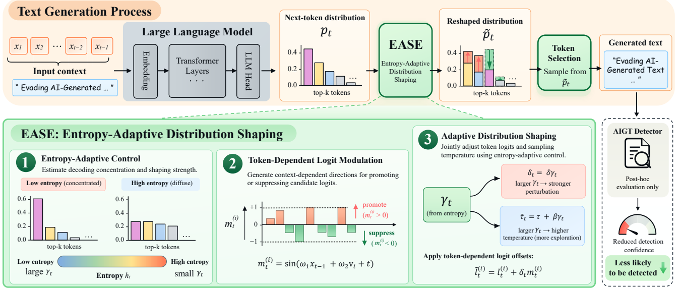
Fig. 2. Overview of EASE. EASE uses top- k predictive entropy to adapt logit perturbation strength and sampling temperature, together with token-dependent logit modulation to reshape the next-token distribution before sampling.
