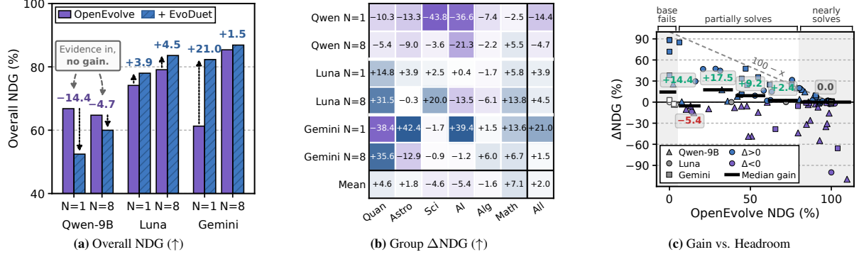
Figure 6: Discovery performance of OpenEvolve with and without EVO DUET. Results cover 21 paired tasks with N = 1 or 8 candidates per iteration. For each model, method, task, and N , we report the best NDG across four runs. (a) Mean best NDG across tasks and the gain from adding EVO DUET ( \Delta NDG). (b) Mean \Delta NDG within each task group. (c) Task-level \Delta NDG versus OpenEvolve’s NDG; black bars and labels show the median gain within each NDG range.
