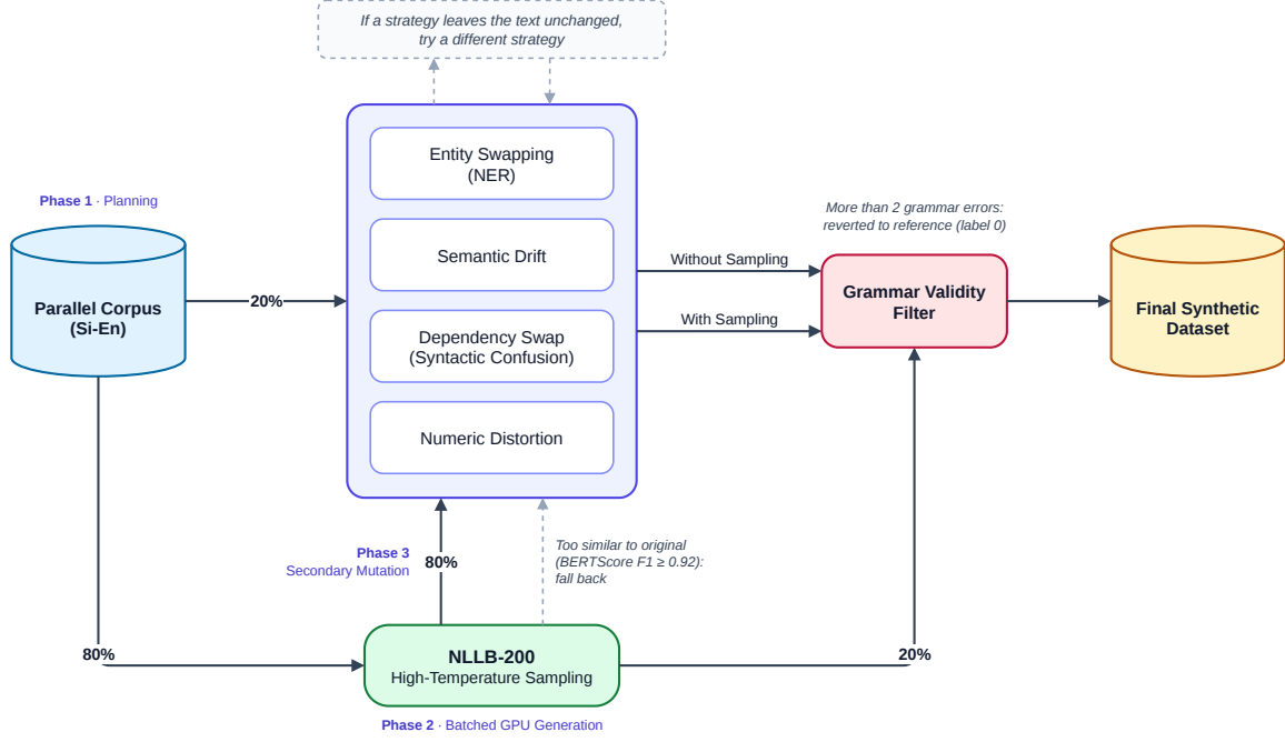
Figure 1: Dataset generation pipeline showing the three-phase probabilistic chain.
