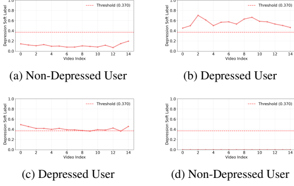
Figure 9: Temporal prediction trajectory of BehavDep.
