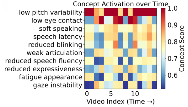
Figure 2: Temporal activation analysis of clinically grounded concepts for a depressed user. The heatmap illustrates the dynamic activation of depression-related behavioral concepts across video segments.
