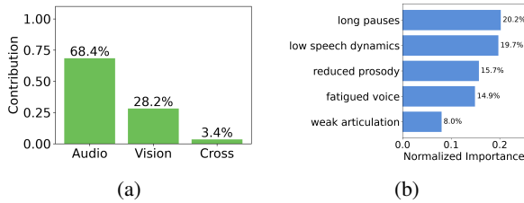
Figure 5: (a) Contribution analysis of different modalities and (b) acoustic feature importance
