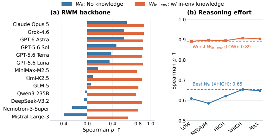
Figure 3: RWM rankings on OLMo3-100M across (a) backbones and (b) Claude Opus 5 reasoning-effort settings.
