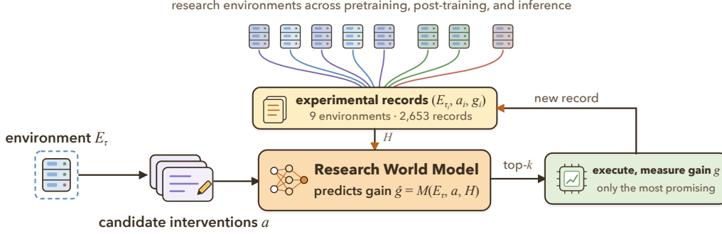
Figure 1: Large language models as Research World Models. Given a research environment E_{\tau} and candidate interventions a , an RWM predicts gains \hat{g} before execution, so that only the most promising interventions consume experimental budget. Executed experiments become records (E_{\tau_i}, a_i, g_i) that form history H for subsequent predictions. Records may come from the same environment or from other environments, allowing the same RWM to serve a target environment that has no records of its own.
