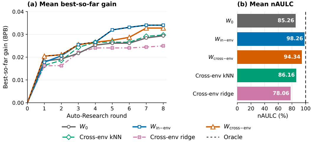
Figure 2: Multi-round Autoresearch on OLMo3-100M. Means over five Autoresearch evaluations, each with eight rounds. (a) Best-so-far gain (BPB). (b) nAULC (%), computed by normalizing each evaluation’s curve area by that of its matched Arrival Oracle and then averaging across evaluations.
