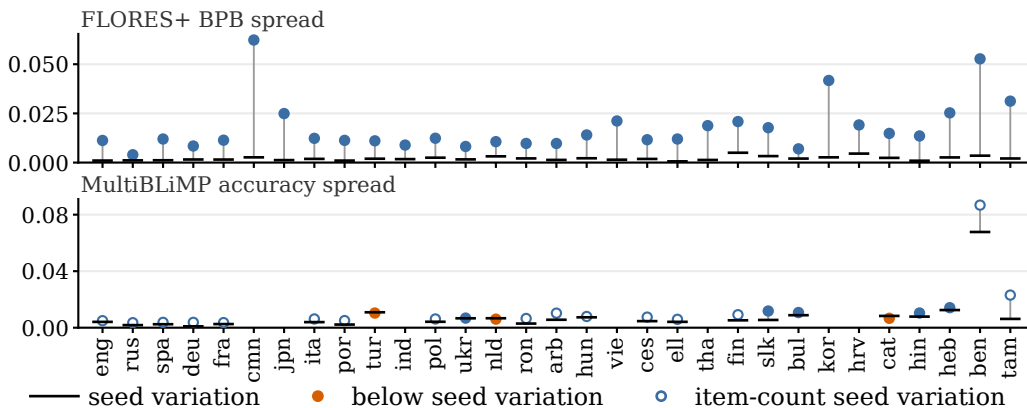
Figure 4: Per-language spread of FLORES+ BPB (top) and MultiBLiMP accuracy (bottom) across the 54 tokenizers, languages in approximately decreasing order of share of the language-model training data (largest at left). Each dot is the standard deviation of the outcome across the 54 tokenizers, and the horizontal tick in the same column, joined to the dot by a thin line, is that language’s seed variation; orange dots are languages where the cross-tokenizer standard deviation does not exceed its seed variation (MultiBLiMP: Catalan, Dutch and Turkish). MultiBLiMP accuracy for a language is estimated from a finite number of minimal pairs, so a fixed model’s measured accuracy varies with a binomial standard error of \sqrt{(p(1-p)/n)} for n pairs. An open dot marks a language for which the pooled seed standard deviation does not exceed this standard error: for these languages, run-to-run variation cannot be measured more finely than the benchmark’s own sampling noise. Languages without MultiBLiMP coverage have no dot in the bottom panel.
