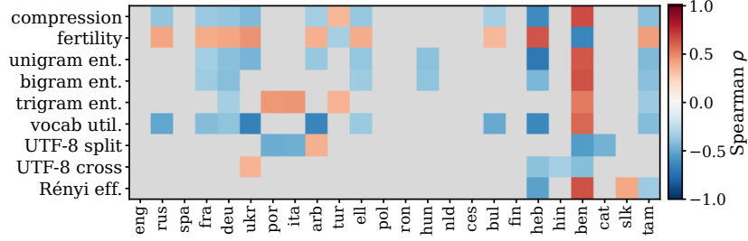
Figure 7: Per-language Spearman \rho between each intrinsic metric (measured on FLORES+ text, as in Fig. 5) and per-language MultiBLiMP accuracy, across the 54 tokenizers, for the 24 covered trained languages ordered from highest to lowest training-data share. The boundary-crossing entries for English and Dutch are undefined (zero variance).
