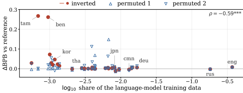
Figure 2: Per-language change in FLORES+ BPB relative to reference (the model trained with the GPT-4o BPE reference tokenizer) for the 31 languages of the training mixture, as a function of the language’s log LM share. Filled circles: inverted-allocation tokenizer, in which languages with the smallest nominal sampling weights in the language-model training data receive the largest tokenizer shares. Open triangles: the two permuted allocation tokenizers, in which the tokenizer shares are assigned randomly.
