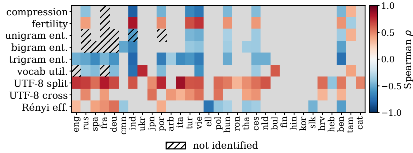
Figure 5: Per-language Spearman \rho between each intrinsic metric and FLORES+ BPB across the 54 tokenizers, for the 31 languages of the training mixture ordered from the highest to the lowest share of it. Only BH-FDR-significant entries are colored. The boundary-crossing entries for English, Indonesian, and Dutch are undefined (zero variance), and the char-split entry for Korean has n = 53 . Hatching marks the 13 entries that are not identified under the measured-composition control of §E, where the metric and the measured number of training bytes of the language correlate at |\rho| > 0.9 across the tokenizer set.
