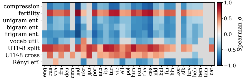
Figure 6: Per-language Spearman \rho between each FineWeb2-measured intrinsic metric and per-language FineWeb2-validation BPB, across the 54 tokenizers, for the 31 trained languages ordered from highest to lowest training-data share. FineWeb2 analogue of Fig. 5.
