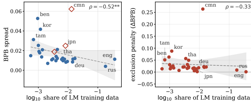
Figure 1: Left: the standard deviation of a language’s FLORES+ BPB across the 54 tokenizers (BPB spread) vs. the language’s log LM share (Spearman \rho = -0.52 , p = 0.003 ). Open diamonds mark the three languages written without word boundaries (Chinese, Japanese, and Thai). Right: the exclusion penalty (defined in the text) against the same axis (Spearman \rho = -0.33 , p = 0.068 ). The horizontal line marks a penalty of zero. Dashed lines are ordinary-least-squares fits, and the grey regions are 95% confidence regions for the fitted mean.
