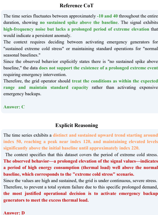
Figure 9 Verbalization bottleneck in CoT reasoning. An operational decision over a temperature series with four choices. CoT (bottom right) runs a CoT trace that first verbalizes the signal as text, then reasons from that textual summary rather than the original representation, and reaches an incorrect final answer. Spans are colored grounded , correct but insufficient , and incorrect .
