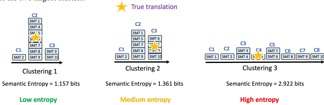
Figure 5: Illustration of semantic-equivalence clusters at different uncertainty levels. Each cluster groups logically equivalent SMT-LIB candidates, and the gold star (★) denotes the ground-truth translation. As entropy increases, the candidates become more evenly distributed across clusters, reducing the reliability of the largest cluster. (a) Low entropy : the largest cluster contains the ground truth; (b) Medium entropy : the ground truth appears in a secondary cluster; and (c) High entropy : the largest cluster is no longer a reliable indicator of correctness.
