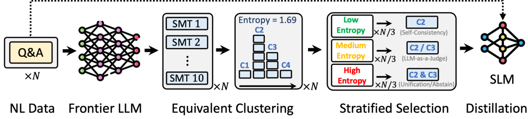
Figure 2: Schematic overview of Stratified Consistency Distillation: For each training sample, we generate 10 SMT-LIB translations using a frontier LLM (e.g., Claude Sonnet 3.7). These translations are clustered based on semantic equivalence, and semantic entropy is computed. The data is then stratified into three groups by entropy: Low entropy : Apply majority voting for self-consistency; Medium entropy : Use LLM-as-a-Judge to select among the top-2 clusters; High entropy : Perform unification of the top-2 translations or abstain the data. Finally, we distill the knowledge into a smaller model (e.g., Qwen) via fine-tuning on Q&A pairs and pseudo-labels derived from stratified selection.
