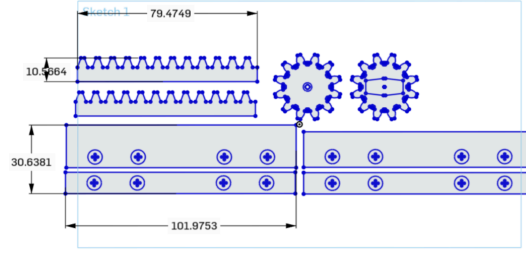
Figure 3: CAD model of rack and pinion mechanism for linear motion conversion
