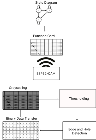
Figure 4: Working flow of Punched Card Reader
