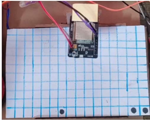
Figure 12: ESP32-CAM image acquisition setup used for punch card digitization
