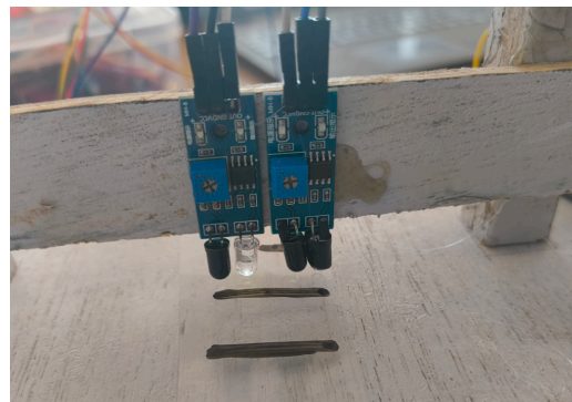
Figure 11: Dual IR alignment for tape symbol detection
