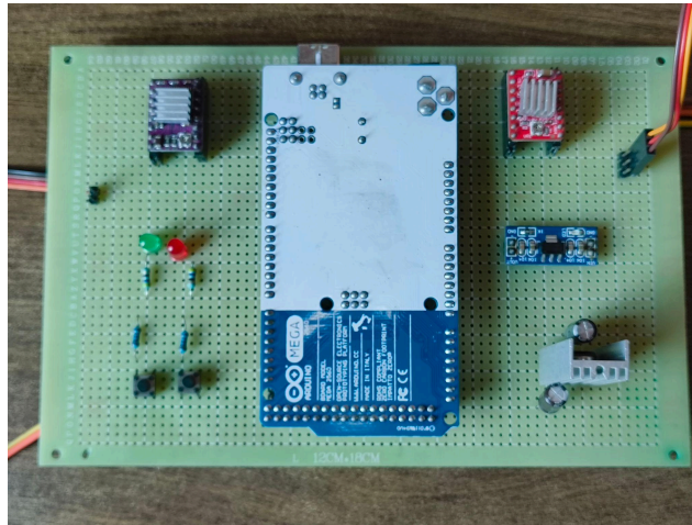
Figure 9: Main Control Board of the System
