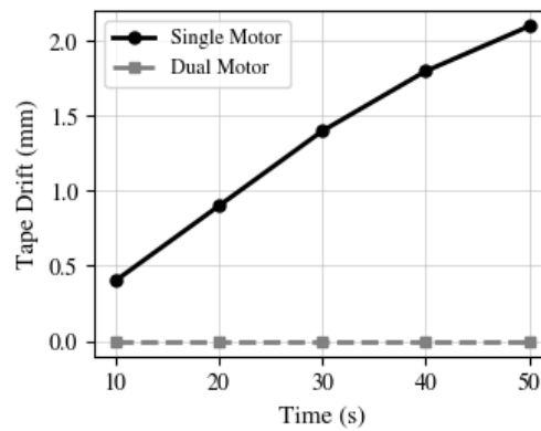
Figure 10: Comparison of tape drift between single-motor and dual-motor tape transport systems
