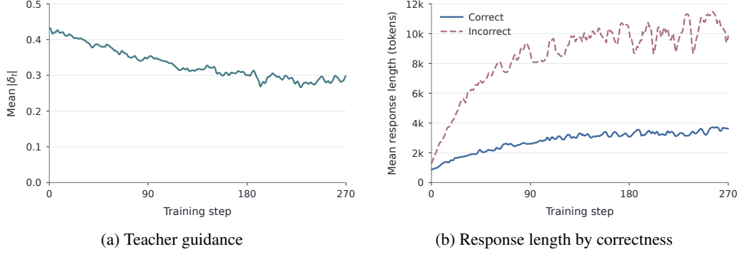
Figure 5: Training diagnostics for the 4B student with RA+REINFORCE++. The guidance weight is fixed at \lambda = 10 , and the horizontal axis counts rollout batches. (a) Recorded mean absolute guidance term |\delta_t| , averaged over the tokens of each batch. (b) Mean response length separated by verifier correctness. The curves are from a single training seed.
