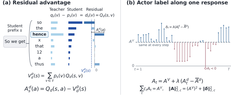
Figure 1: Local teacher guidance redistributes the verifier’s response-level credit. (a) At one prefix, the reward Q_d(s, v) = q_s(v) - p_s(v) over the student’s likeliest tokens, its value V_d^p(s) under the student policy, and the advantage A_s^d(a) of the sampled token, here the student’s third choice and the teacher’s first. (b) Labels along one response, with blue and coral stems for positive and negative guidance terms \delta_t ; each label is A^V plus a centered guidance term, so the labels’ weighted mean is A^V .
