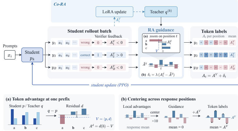
Figure 2: One iteration of RA and Co-RA. Three schematic responses, only the middle one correct, receive verifier advantages A_i^V . RA adds a centered guidance term to every token label. Token strips show one cell per position, blue for A_t > 0 and rose for A_t < 0 , darker for larger |A_t| ; the last cell is the response mean, which centering pins to A_i^V . Insets show (a) the student value baseline at one prefix and (b) response centering. In Co-RA, a LoRA adapter on the frozen teacher is trained with the verifier advantages of the same scored batch and supplies the next iteration’s residual.
