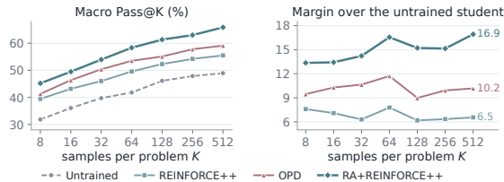
Figure 6: The margin over the untrained student does not close up to Pass@512. Macro Pass@K of Table 28 and each trained run’s margin over the untrained student, in points.
