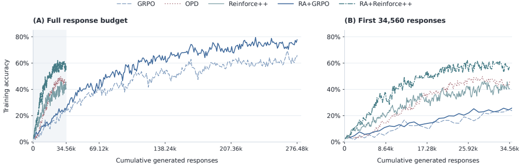
Figure 4: Training accuracy of Qwen3-4B-Base on DAPO-Math-17K. (A) Full two-epoch response budgets: 276,480 generations for GRPO runs and 34,560 for the one-response runs. (B) The first 34,560 generations, the shaded region in (A), show the early trajectories at the same response budget. Curves show logged training accuracy; Co-RA is omitted.
