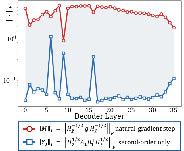
Figure 2: Layer-wise whitened Frobenius norms of the Stage-1 adapter, \|Y_0\|_F = \|H_z^{1/2} A_1 B_1^\top H_{\hat{x}}^{1/2}\|_F (blue; the second-order compensation), and of the natural-gradient step on the compensated model, \|M\|_F = \|H_z^{-1/2} g H_{\hat{x}}^{-1/2}\|_F (red). Both are expressed in the whitened coordinates induced by the curvature metric of Eq. (2), so their magnitudes are directly comparable; each point averages the seven linear modules of a decoder layer, and the vertical axis is logarithmic. The natural-gradient step is larger in every layer, indicating that the second-order objective alone leaves substantial loss-sensitive information unexploited. Measured on Qwen3-4B quantized to 2 bits with QuIP#, using 16 \times 512 = 8,192 WikiText-2 training tokens and one forward and backward pass per block.
