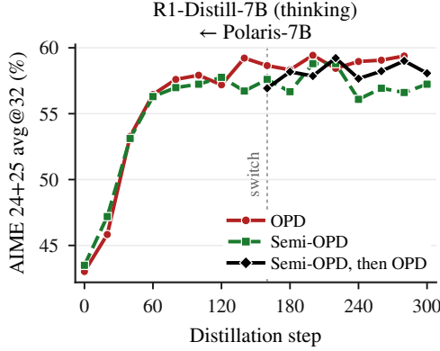
Figure 10 | Switching from Semi-OPD to OPD on a high-overlap pair with an initial top-64 overlap ratio of 86.8% closes the gap with OPD applied from scratch.
