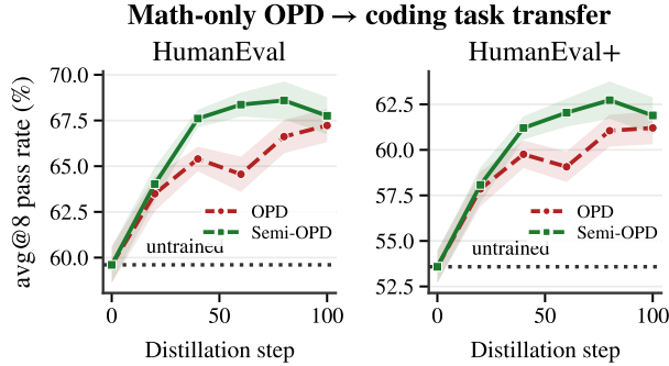
Figure 11 | Transfer to coding. Code performance of models distilled on math only (Qwen3-1.7B ← Qwen3-4B-Instruct-2507).
