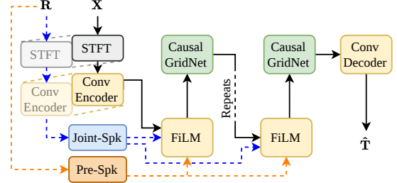
Fig. 2. System architecture for \mathcal{M}_{\text{MSX}} . The enrolment speech \mathbf{R} can be processed by a jointly-trained speaker encoder (Joint-Spk) or a pre-trained speaker encoder (Pre-Spk).
