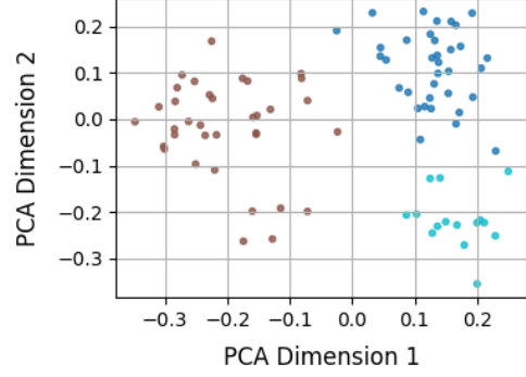
Figure 4: PCA projection of training example embeddings on GSM8K using the gtr-t5-base encoder. We cluster 85 training examples into k = 3 semantic groups using k-means.
