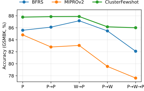
Figure 2: Accuracy across BetterTogether strategies on GSM8K using Qwen2.5-7B-Instruct.
