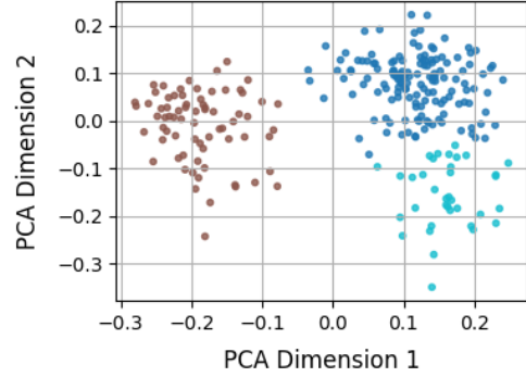
Figure 5: PCA projection of 250 validation example embeddings on GSM8K using the gtr-t5-base encoder.
