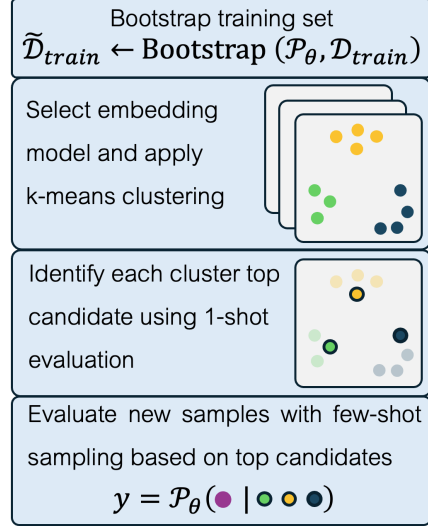
Figure 1: An illustration depicting ClusterFewshot approach for bootstrapped demonstrations.
