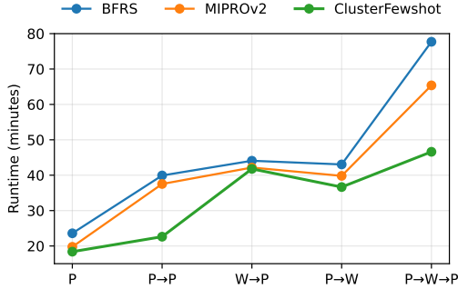
Figure 3: End-to-end runtime across BetterTogether strategies on GSM8K using Qwen2.5-7B-Instruct.
