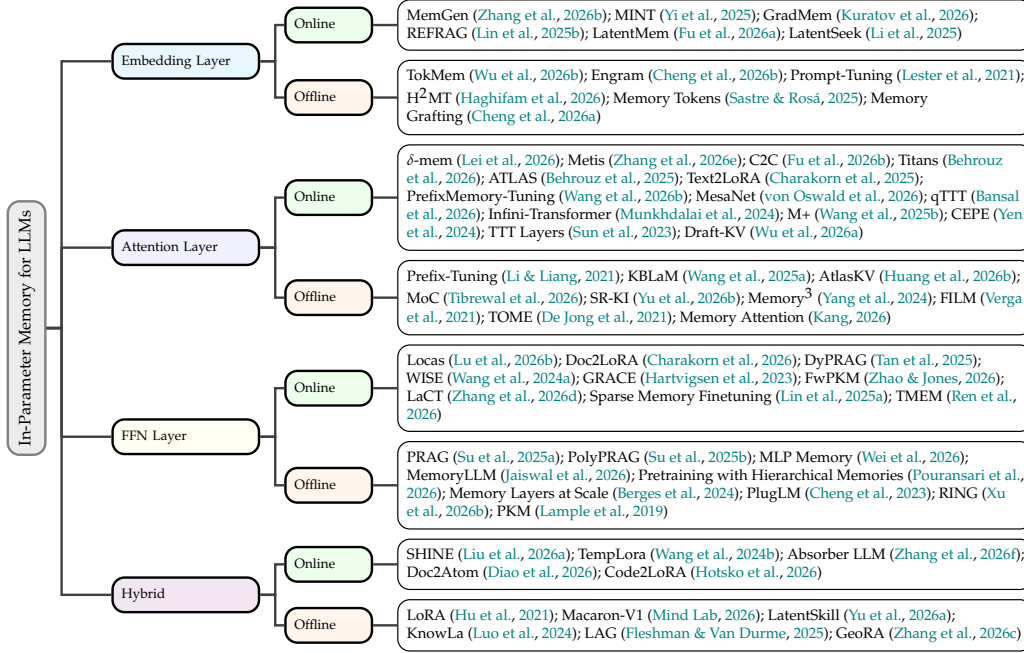
Figure 3: Overall taxonomy and representative methods of IPM for LLMs.
