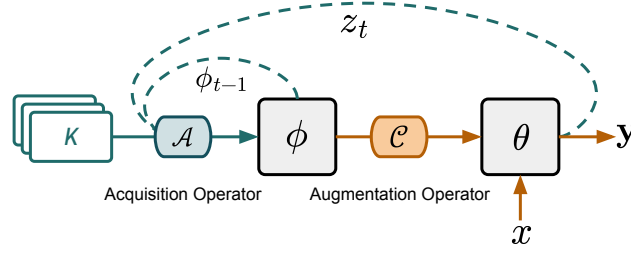
Figure 2: A demonstration of the operator formulation of in-parameter memory.
