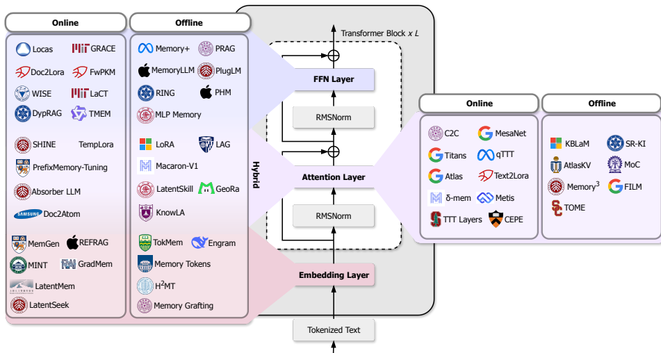
Figure 1: A demonstration of the representative methods in the two-dimensional taxonomy.
