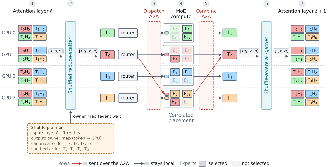
Fig. 5: Token shuffling end to end. After the attention of layer \ell ①, the shuffle planner predicts each token’s owner rank from its layer- (\ell-1) routes, and the shuffled reduce-scatter ② delivers each row to that rank. The dispatch ③, the expert computation ④ and the combine ⑤ then find most of the token’s experts local. The shuffle-aware all-gather ⑥ restores canonical order before the next attention block ⑦.
