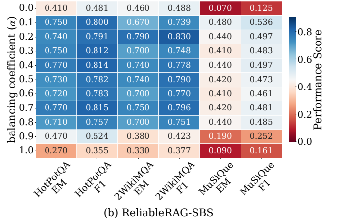
Figure 4: EM and F1 performance of ReliableRAG across various configurations of the balancing coefficient \alpha that regulates the dual-factor perception mechanism within the Triple Evaluation module. Results compare (a) ReliableRAG-TBS and (b) ReliableRAG-SBS variants, evaluated under the ideal setting using the dev sets of three multi-hop QA datasets.
