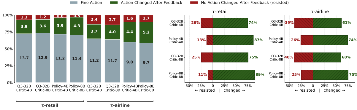
Figure 8: Left: Distribution of tool-calling agent actions across different agentic scenarios. Right: Comparison of how often instruct and CATC agents resist the verification signal after receiving critique feedback.
