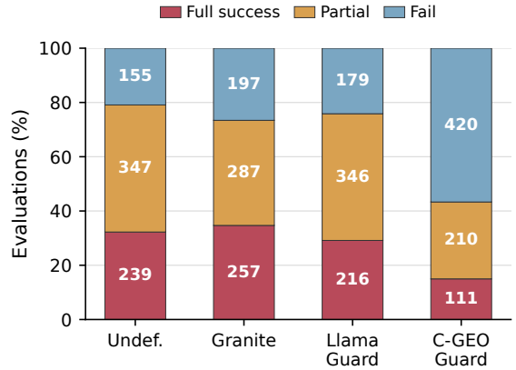
Figure 4: Pooled ASR outcome distribution across three victim LLMs ( N=741 per defense). C-GEO Guard shifts the majority of outcomes from full/partial success to fail. NeMo excluded (Llama-4 unusable).
