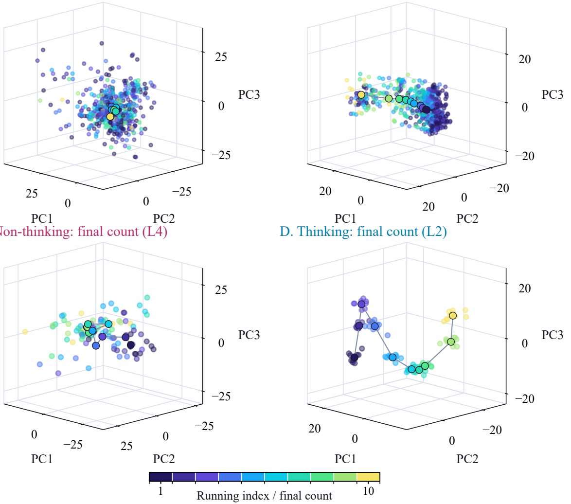
Figure 38: Count geometry. Cross-validated NCC selects L2/L4/L4/L2 for A/B/C/D. Separate PCA projections show 550 running index states (A/B) and 100 answer states (C/D) per mode. Out-lined class means are connected in label order. The three components explain 50.9/48.1/74.0/71.7% of selection variance in A/B/C/D. All panels use the same camera view and equal coordinate units within each panel.
