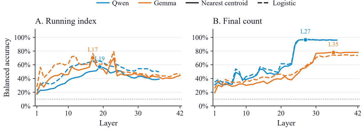
Figure 23: Count readout across layers. A. Running index at trace-item endpoints. B. Final count at the answer query. Both analyses cover N = 1-10 . Curves pool predictions from five seed-grouped cross-validation folds (20 seeds/model): 1,107 Qwen/1,045 Gemma running states and 200 answer states each. Solid/dashed curves denote NCC/logistic classifiers; labeled markers identify NCC-selected layers. Blue denotes Qwen and orange Gemma; dotted lines mark 10% chance.
