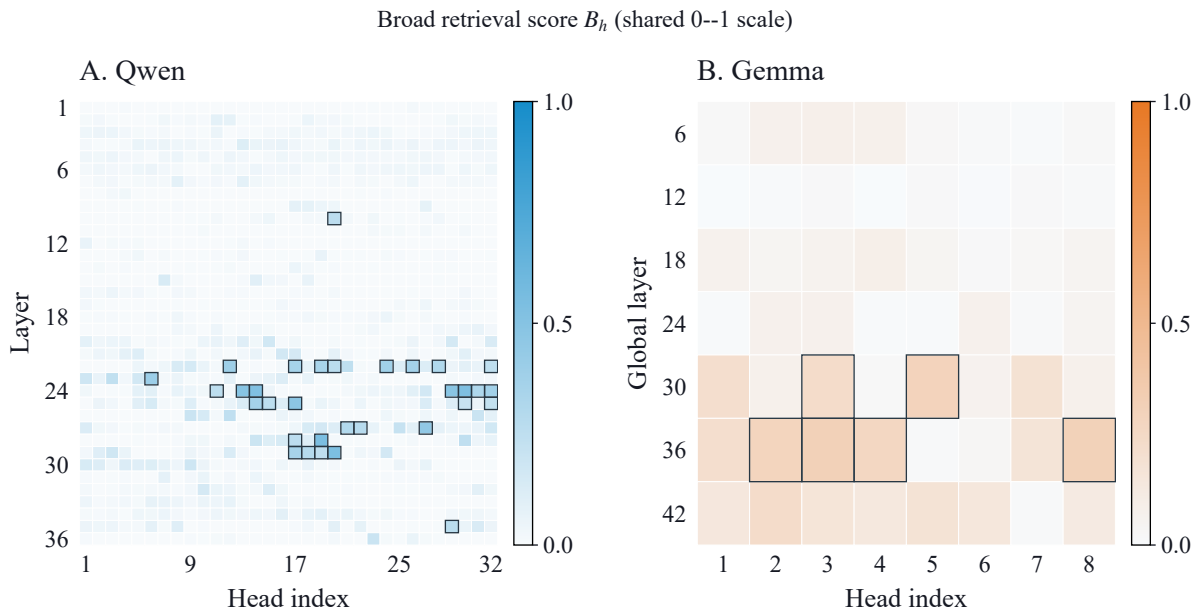
Figure 15: Complete broad-retrieval scores. A. All 1,152 Qwen heads. B. All 56 Gemma global-attention heads. Cells show mean B_h on 180 selection prompts. Horizontal axes show heads; vertical axes show layers from shallow to deep. Both panels use a linear 0–1 scale. Outlines mark frozen Qwen Top-32/Gemma Top-6 membership.
