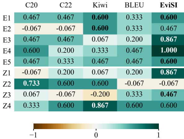
Fig. 3. Kendall \tau_b with human rankings across six systems in each corpus, with a fixed [-1, 1] scale. Bold marks row maxima, including ties. C20/C22: COMET20/22; Kiwi: COMETKiwi; BLEU: Sentence BLEU. All corpora, including negative results, are shown.
