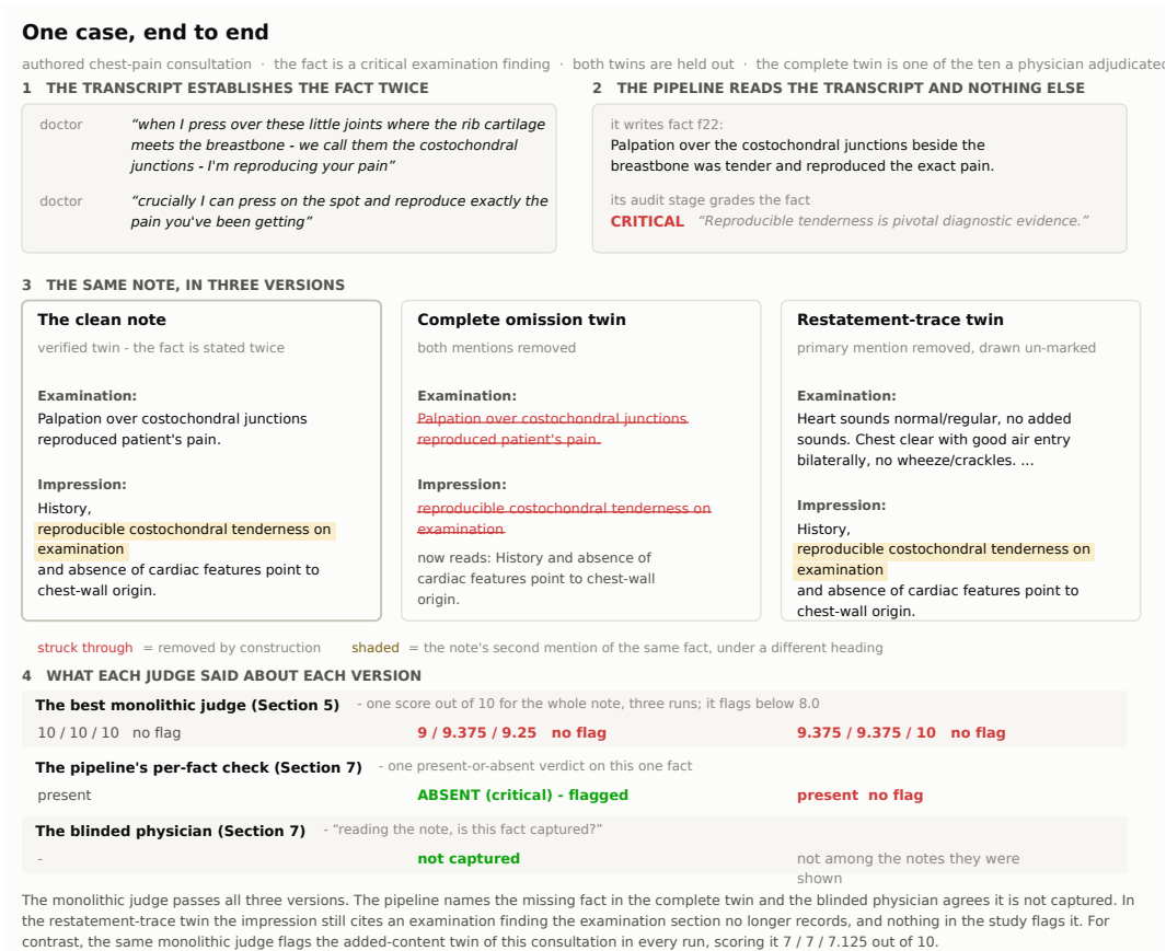
Figure 1: One case end to end: a critical examination finding the transcript establishes twice, the note records twice, and two twins remove differently. The monolithic judge passes all three versions; the pipeline’s per-fact check names the missing fact in the complete twin and the blinded physician agrees it is not captured. The restatement-trace twin is drawn un-marked, as a reader sees it: the examination reads normally, the impression still cites the finding it no longer records, and nothing in the study flags it. Each note column is abridged to the passages the fact lives in, and the twins differ from the clean note by deletion only. The case is an authored consultation, so the figure excerpts only our own transcript and notes and no vendor text appears anywhere.
