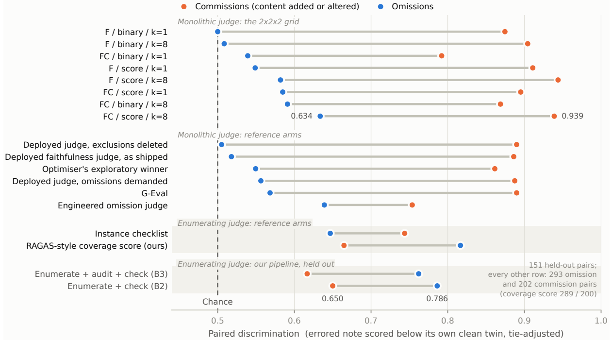
Figure 4: Paired discrimination on omissions against commissions, per judge design. The measure is the tie-adjusted probability that the errored note scores strictly below its own clean twin, plus half the tie mass; chance is 0.500. The sets: the monolithic and reference-judge rows are the 495 evaluation pairs over 112 consultations (293 omissions, 202 commissions; the eight designs at 3 replicates, reference judges at 2), and the two pipeline rows are the 151 held-out confirmation pairs over 47 consultations (131 omissions, 20 commissions), means over 3 replicates. The coverage-score row is the one exception to those counts: its paired values rest on 289 omission and 200 commission pairs per replicate, because parse failures cost that arm 14 of its 1,214 records. Design codes read as criterion / answer format / sample count for the designs Section 4 describes in words; the released data spells them F-bin-k1 to FC-score-k8.
