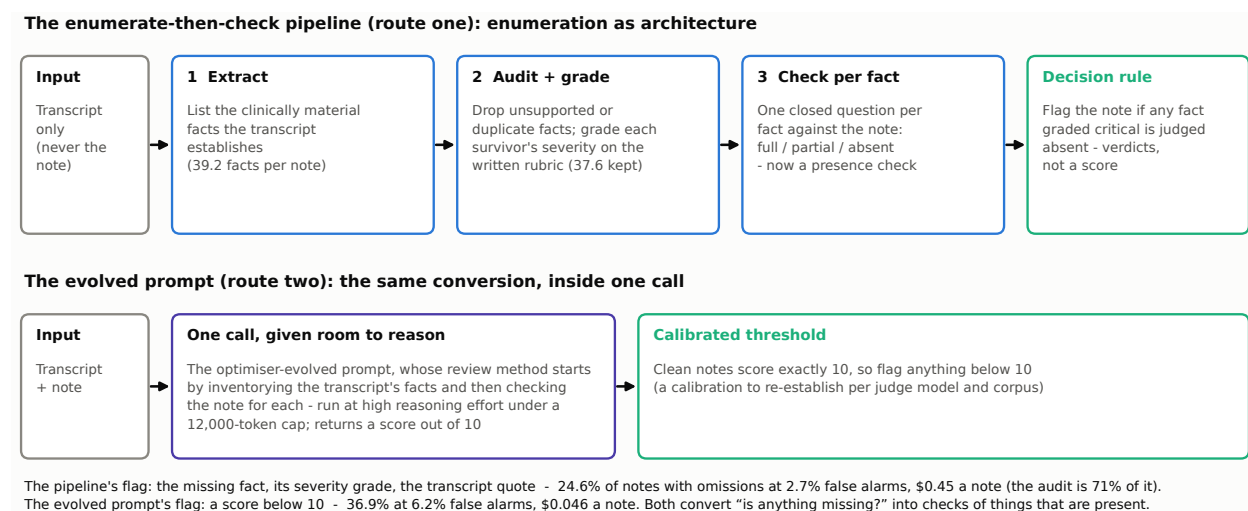
Figure 6: The two methods, as run. The enumerate-then-check pipeline (route one in the released data) converts the absence question into presence checks in the architecture: an extraction call that never sees the note, an audit that drops weak facts and grades the rest, one closed check per fact, and a decision rule over the verdicts. The lane draws the three-stage tier, the only one whose audit grades severity and so the only one the decision rule can be stated on; the two-stage tier stops after the per-fact check and carries the higher paired score. The three-stage tier also runs a second look over the facts the check called absent, which the lane does not draw (Appendix C). The evolved prompt (route two) makes the same conversion inside one call: a GEPA-evolved prompt whose review method starts by inventorying the transcript’s facts and then checking the note for each, executed at high reasoning effort and read through a clean-note calibration. Operating points are the evaluation-set figures of Table 8 and prices those of Table 9; the fact counts inside the pipeline’s lane are the held-out confirmation run’s, 39.2 facts extracted per note and 37.6 left after the audit.
