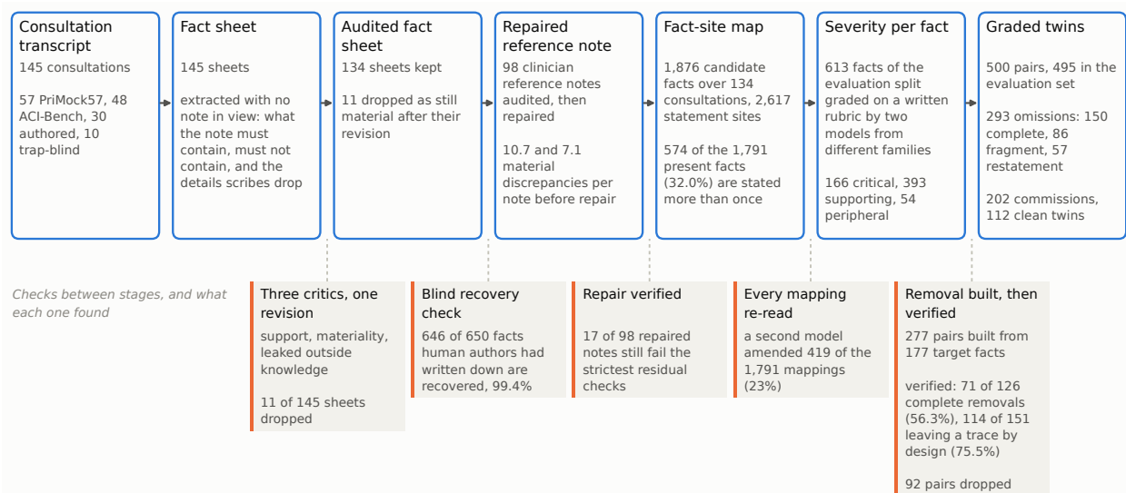
Figure 2: The answer key is built from the transcript, not borrowed from the reference note. Each box is a construction stage and carries what it produced; each chip below is the check that stands between two stages, and what that check found or rejected. The trap-blind stratum in the corpus band is authored consultations written with no knowledge of the benchmark’s trap schema, as a representativeness guard. Severity is graded per fact by two models from different families on a written rubric; they split on 93 of the 613 facts, and the lower grade is taken. The two checks that carry findings of their own are blind recovery, where extraction recovers 646 of 650 facts that human authors had written down for the same consultations, and removal verification, where only 71 of 126 attempts to remove every trace of a fact from a real note survive a cross-family panel against 114 of 151 for removals that leave a trace by design.
