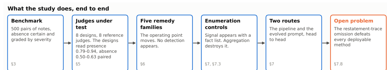
Figure 3: The experimental programme in one line. The benchmark of Section 3 feeds an eight-design ablation and eight reference judges (Section 5, the asymmetry); five remedy families fail to restore single-note detection (Section 6); two enumeration controls locate the mechanism (Section 7, Section 7.3); two methods implement the conversion of absence into presence checks and are compared head to head (Section 7); and one case defeats every deployable method (Section 7.8). Counts, where a box carries them, are the pairs or designs involved.
