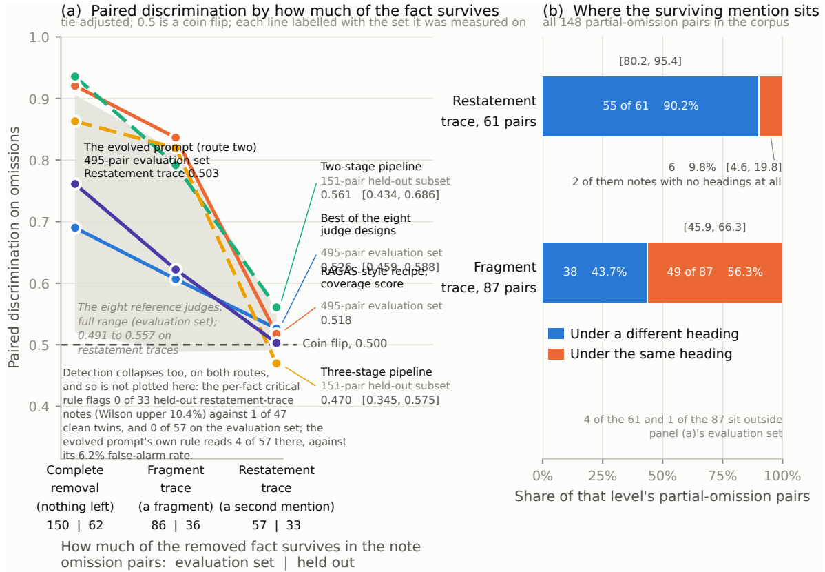
Figure 8: Every method we measured in the primary judge family collapses on the omission whose restatement survives elsewhere in the note, and the supply of those cases says why. (a) Paired discrimination on omissions - how often a note carrying an omission scores below its own verified-clean twin, tie-adjusted, where 0.5 is a coin flip - split by how much of the removed fact survives: nothing (complete removal), a fragment of it (fragment trace), or an explicit or closely paraphrased second mention (restatement trace). Each line names the set it was measured on, and the two sets are read separately rather than ranked against each other: the best of the eight judge designs, the range across the eight reference judges, the RAGAS-style recipe (our implementation, read as its coverage score rather than at its own flag-everything rule), and the evolved prompt (route two in the released data, the optimiser’s winner at reasoning effort high, three replicates averaged) are measured on the 495-pair evaluation set, whose 293 omission pairs split 150 / 86 / 57 across the three levels; the two-stage and three-stage pipelines are measured on the 151-pair held-out subset, whose 131 omission pairs split 62 / 36 / 33. The band spans all eight reference judges, the coverage recipe among them at the aggregate score it ships, so that recipe appears twice: once inside the band and once as its own line at the coverage component alone. The coverage recipe is also the one line with denominators of its own, 148 / 84 / 57, because parse failures cost it 14 of its 1,214 records. The interval printed beside each restatement-trace value is a 95% bootstrap interval over consultations, computed over 35 consultations for the evaluation-set line that carries one and 20 for the held-out ones, and every one of them contains 0.5; the coverage recipe’s and the evolved prompt’s restatement-trace values have no such interval in the released artefacts and are quoted as point estimates. Detection collapses with discrimination, and is annotated rather than plotted because it is a rate at a rule rather than a discrimination score: the per-fact rule flags 0 of 33 held-out restatement-trace notes against 1 of 47 clean twins, 0 of 57 on the full evaluation set against 3 of 112, and the evolved prompt’s own rule reads 4 of 57 there against its 6.2% false-alarm rate. (b) Where the surviving mention sits, over all 148 partial-omission pairs in the corpus (61 restatement-trace, of which 57 are in the evaluation set, and 87 fragment-trace, of which 86 are): in 55 of 61 restatement-trace pairs, 90.2% [80.2, 95.4], the survivor sits under a different heading from the instance that was removed, while 49 of 87 fragment-trace pairs, 56.3% [45.9, 66.3], keep it under the same heading; two of the six same-heading restatement traces are notes with no headings at all. Reading: once a restatement trace survives, every method plotted here sits at or below its own noise floor. The one exception the study holds is not plotted - the second judge family’s checker discriminates the class at 0.636 paired while the rule still catches none (Section 7.8). The supply explains why - a restatement trace is almost always a different-heading survivor, recoverable only by reading the note end to end.
