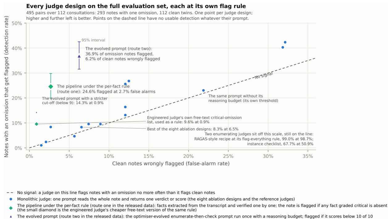
Figure 5: Every judge design at its own flag rule: the levers slide a point along the no-signal line, and only the two methods leave it. Across, how often a judge wrongly flags a clean note; up, how often it flags a note that really carries an omission. A useful detector sits high and to the left; the dashed diagonal is no signal, a judge that flags both kinds of note equally often. Every design is on the 495-pair evaluation set (293 notes with one omission, 112 clean twins; the eight designs pooled over three replicates, 879 and 336 records, the reference judges over two, 586 and 224, and the two method points note-level), each at its own flag rule - fixed before the run for the eight designs and the reference judges, established post hoc for the two methods' rules (Sections 7.5 and 7.6). The eight designs and the deployed-judge wordings sit on or beside the line, and the levers of Section 6 only slide a point along it. Two points sit well clear of it, each with a 95% whisker on its detection rate: the pipeline under the per-fact rule (route one in the released data), at 24.6% detection on 2.7% false alarms, and the evolved prompt (route two), at 36.9% on 6.2%. Three further points are labelled for reference: the evolved prompt with a stricter cut-off, the same prompt run without its reasoning budget, and the engineered judge's own free-text critical-omission list read as a rule. Two enumerating judges flag almost every note and so fall outside the plotted range; their rates are printed inside the figure. Every unlabelled point's values are in Table 4, Table 5 or Table 8; how the pipeline's flag is made from its verdicts is Figure 7.
