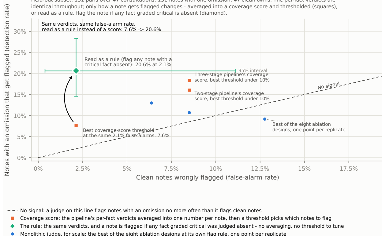
Figure 7: The same per-fact verdicts, turned into a note-level decision two ways. A pipeline that returns one verdict per fact still has to decide, per note, whether to flag it. On the 151-pair held-out subset (131 notes with one omission, 47 clean twins) the three-stage pipeline's verdicts are read two ways with nothing else changed. Averaged into a coverage score and thresholded at the rule's own 2.1% false-alarm rate, they detect 7.6% of the notes with an omission; the best threshold inside a 10% false-alarm budget reaches 18.3% at 8.5% for the three-stage tier and 16.0% at 8.5% for the two-stage tier. Read as the rule - flag the note if any fact graded critical is judged absent - the identical verdicts detect 20.6% at 2.1% (the plotted rule point is replicate 1 of three; across the three the detection reads 20.6, 22.9 and 21.4%, with the false-alarm rate identical in every one). The best of the eight ablation designs is drawn for scale at its own rule, one point per replicate. The identical verdicts, read as a rule rather than averaged into a score, give 2.7 times the detection at the same false-alarm rate.
