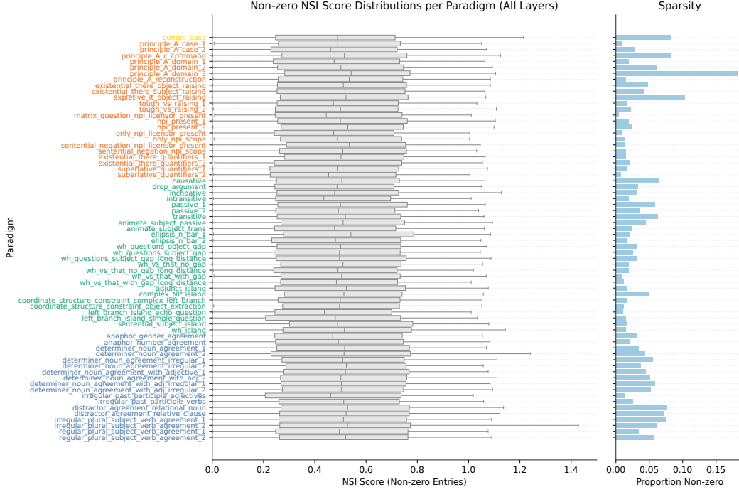
Figure 11: Left: Distributions of non-zero NSI scores (i.e., over sensitive neurons with NSI > 0 ) aggregated across all layers, shown separately for each paradigm. Across paradigms, the mean NSI is typically around \sim 0.5 , indicating that most sensitive neurons exhibit only weak separability. Right: Paradigm-wise proportion of sensitive neurons across all 68 BLiMP/COMPS paradigms for Qwen3-0.6B.
