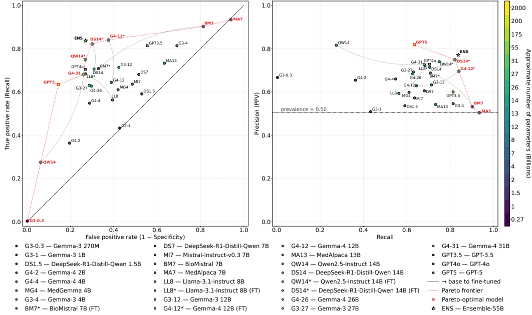
Figure 3: Operating points of all evaluated models in ROC (left) and PR (right) spaces on ECGQuest. As each model make hard true/false decisions, it contributes a single operating point rather than a curve. Marker color encodes the approximate parameter count; circles denote open source models and crosses closed source models. Grey arrows connect each base model to its fine-tuned counterpart (FT), red dashed lines trace the Pareto frontier, and red rings mark Pareto-optimal models. The black dashed lines indicate chance performance.
