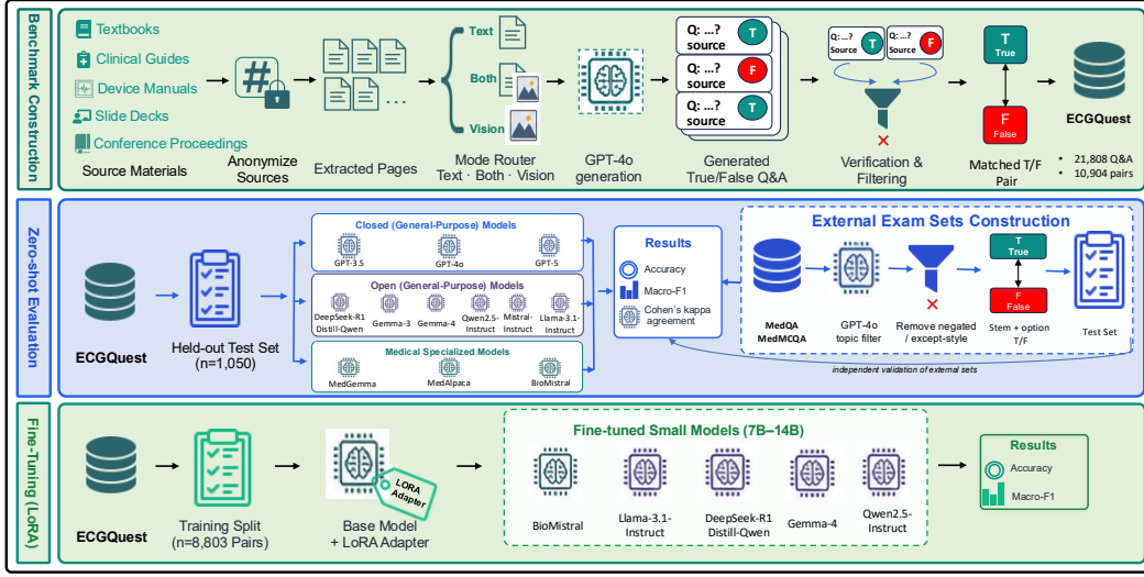
Figure 1: Overview of ECGQuest creation framework. (1) ECG reference materials were anonymized, split into pages, routed by content to a text or vision-based generation model for text extraction, and passed to GPT-4o to generate paired True/False questions. (2) Closed, open, and medically specialized models were tested on the held-out test set ( n=1,050 ), and external ECG-focused MedQA and MedMCQA questions, extracted by GPT-4o ECG-topic filtering and converted to True/False for independent validation. (3) small open models (7–14 B parameters) were fine-tuned with LoRA adapters and re-evaluated.
