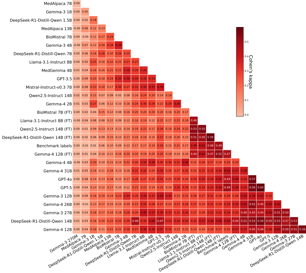
Figure 2: Pairwise Cohen’s \kappa agreement between model predictions and the benchmark reference labels, computed on the held-out benchmark test set ( n = 1,050 ). Higher values (darker) indicate stronger agreement. Values quantify agreement with the benchmark rather than clinical correctness.
