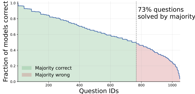
Figure 4: Question-level difficulty/clarity profile on the ECGQuest test set ( n = 1,050 ). Questions are ordered from easiest/clear to hardest/ambiguous according to the fraction of evaluated models that answered each question correctly. The green region represents questions answered correctly by at least half of the models, while the red region represents questions answered correctly by fewer than half of the models. The dashed vertical line indicates that approximately 73% of the questions were answered correctly by at least half of the evaluated models.
