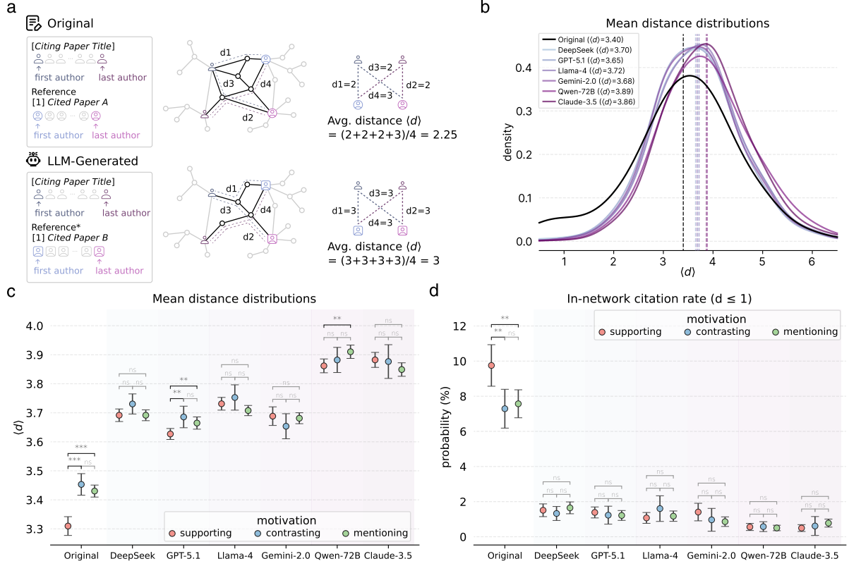
Figure 4: Author-dyad coauthorship distance separates human from LLM citation behavior. (a) For each masked slot, focal and cited first/last authors are resolved to researcher IDs and BFS shortest-path distance computed on a 20.3M-edge, 2.1M-researcher 2015–2024 coauthorship network; per-context mean \langle d \rangle is the unit in (b)–(c). (b) Density of \langle d \rangle : humans peak near 3.4 with a close-circle shoulder; LLMs shift right (3.65–3.89). (c) \langle d \rangle by intent (mean \pm 95% CI; Mann–Whitney U). Humans show drastic gradient, supporting closer than contrasting/mentioning ( p < 0.001 ); LLMs cluster within \pm 0.05 hops. (d) In-network citation rate ( d \leq 1 ). Humans reach 7–10%, elevated for supporting (9.8% vs. 7.3%/7.6%; p < 0.01 ); every LLM stays below 1.6% with no intent gradient.
