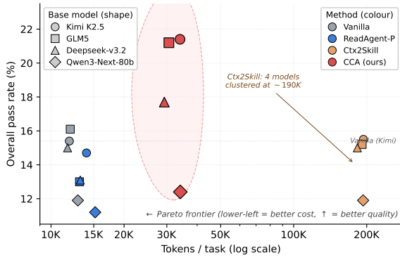
Figure 2: Cost–quality tradeoff for the 16 (method, model) cells of Table 1. Tokens per task on log x ; Overall pass rate on y . CCA (red) dominates the upper-middle Pareto frontier : at \sim 3\times Vanilla’s tokens it adds +6.0/+5.1/+2.7/+0.5 pp on Kimi/GLM-5/DeepSeek/Qwen3 (last is capacity-bounded; see §5.3). Ctx2Skill is the counter-example— \sim 5.7\times CCA’s cost, near-Vanilla pass rate—the lossy-abstraction failure of §5.2. A cost-conscious CCA variant (no R-2; +4.72 pp at \sim 22.7 K tokens) sits further left; see Appendix H.
