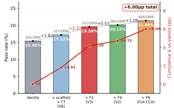
Figure 3: Cumulative buildup from Vanilla to Full CCA on Kimi K2.5 (full 1,899 tasks). The bar+line combo packs four quantities into one view, one per column of Table 3: (i) bar height = pass rate at each configuration; (ii) bar-top label = absolute pass count out of 1,899; (iii) annotations between bars = marginal \Delta pp from adding one feature on top of the previous configuration (F2 highlighted in red as the largest single jump, +2.37pp); (iv) red diamond line on the right axis = cumulative \Delta vs Vanilla , sweeping from 0 to +6.00pp as features are added. Build-up path: Vanilla \rightarrow V6 \rightarrow V3 \rightarrow V2 \rightarrow Full; the four marginal \Delta pp annotations sum exactly to +6.00pp.
