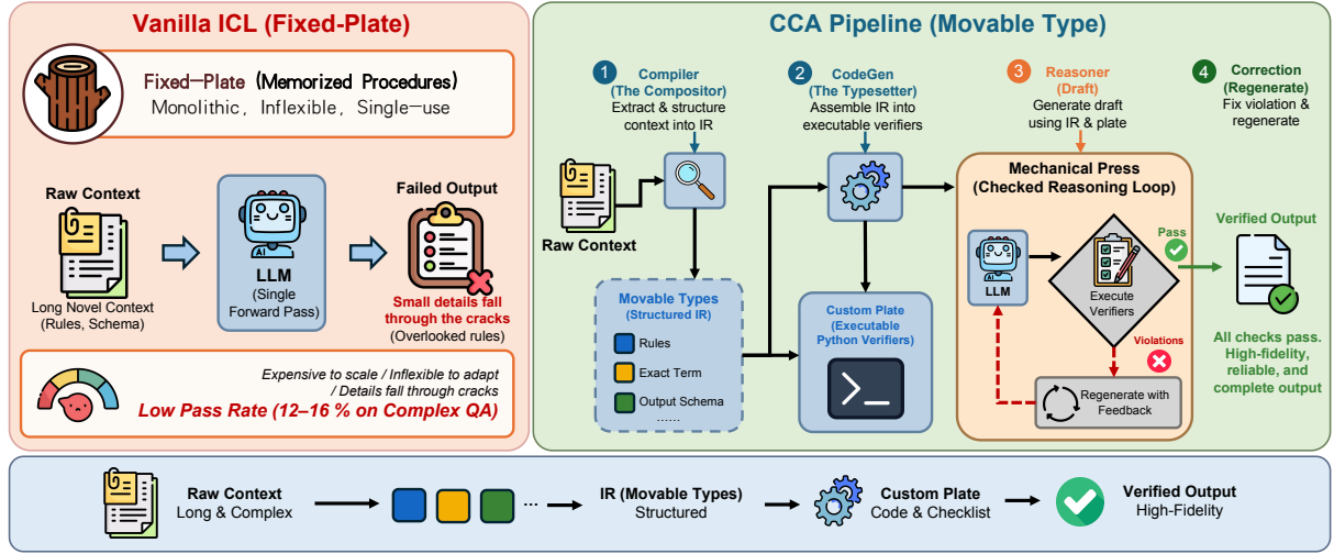
Figure 1: CCA pipeline vs vanilla ICL. Left (red, “Fixed-Plate”): vanilla ICL pushes the long context through a single LLM forward pass; small details fall through the cracks and pass rate stays at 12–16% on rubric-graded benchmarks (Table 1). Right (green, “Movable Type”): CCA decomposes the context into reusable typed pieces in four stages—(1) Compiler (the compositor) extracts a JSON IR of rules, exact terms, workflow, and output schema (F1); (2) CodeGen (the typesetter) assembles up to three Python verifiers from the IR (F3, F5); (3) Reasoner drafts an answer using the IR as an explicit checklist (F2); (4) Correction regenerates with violation feedback when verifiers flag \geq 2 violations (F4, F6). Per-context artifacts (stages 1–2) are amortized over every question sharing the context; per-task stages (3–4) run once per question. Head/tail context truncation (F7) is described in §3. The pipeline converts the diffuse self-judgment “did I remember everything?” into the mechanical check “did my code-verifier pass?”.
