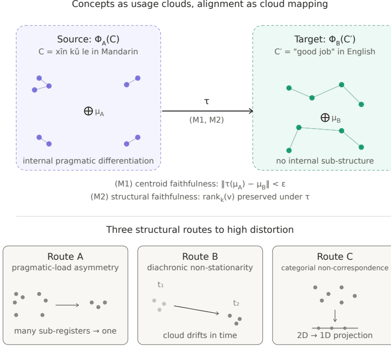
Figure 1: Concepts as usage clouds, alignment as cloud mapping (visualization of the framework introduced in §3). Top : a source cloud \Phi_A(\text{xin ku le}) exhibits internal pragmatic differentiation, with four sub-regions corresponding to superior-to-subordinate, peer-to-peer, service-encounter, and ironic uses; the target cloud \Phi_B(\text{good job}) has no corresponding sub-structure. The alignment map \tau is judged on two conditions: (M1) centroid faithfulness, \|\tau(\mu_A) - \mu_B\| < \varepsilon , and (M2) structural faithfulness, preservation of \text{rank}_k(v) under \tau . Even when \tau satisfies (M1) by aligning centroids, (M2) is necessarily violated when the target lacks the source’s pragmatic dimensionality. Bottom : the three structural routes to a large infimum in Definition 3. Route A (pragmatic-load asymmetry): many sub-registers in the source collapse to one in the target. Route B (diachronic non-stationarity): the cloud drifts across time windows t_1 \rightarrow t_2 , so no synchronic gloss can simultaneously match both. Route C (categorical non-correspondence): the target cloud is a projection of the source onto a lower-dimensional subspace.
