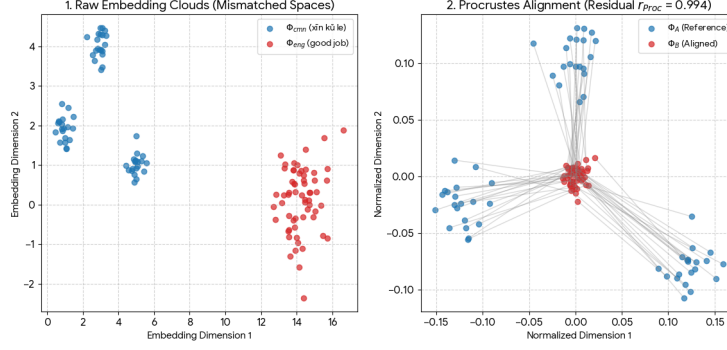
Figure 2: Illustrative example with synthetic clouds: the Procrustes residual r_{Proc} (Metric 3, Manifold-Curvature Mismatch) for a structured source cloud and a flat target cloud. Left : the raw usage clouds \Phi_{cmn}(x\bar{n} k\ddot{u} le) (blue), partitioned into distinct pragmatic regions (superior-to-subordinate, peer-to-peer, service encounter), and \Phi_{eng}(good job) (red). Right : the clouds after optimal Procrustes alignment (translation, rotation, and scaling); gray lines connect corresponding points. r_{Proc} is the sum of squared distances between corresponding points after alignment. Even the best linear map cannot stretch the flat target cloud over the sub-clusters of the source cloud, so r_{Proc} remains high: the internal rank structure and local neighborhood densities are incompatible, an (M2) violation.
