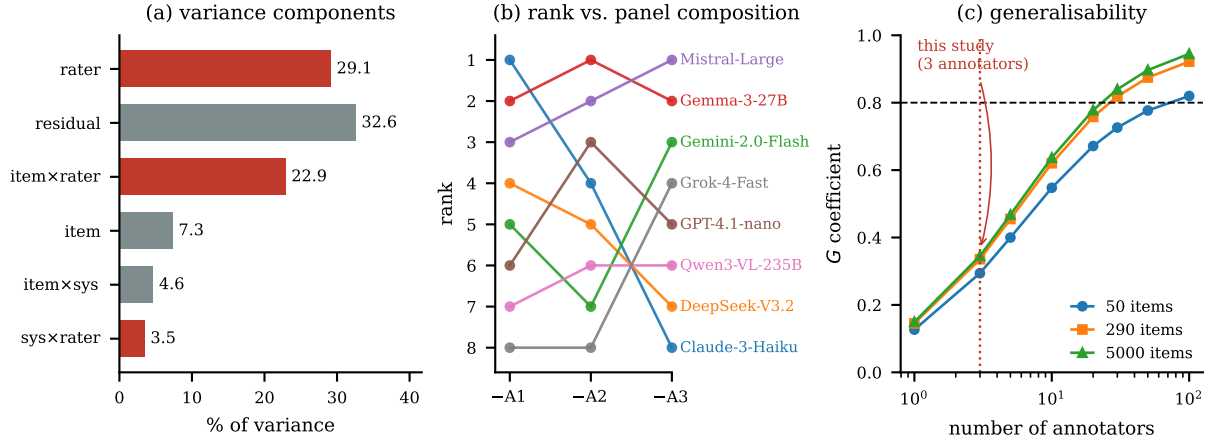
Figure 1: (a) Random-effect variance components; annotator-related terms (red) dominate. The system is a fixed factor and accounts for 0.7% of the total sum of squares against 22.1% for the annotator main effect. (b) System rank as a function of which annotator is excluded. (c) Decision study: G saturates in the number of items, so three annotators cannot reach G = 0.8 at any corpus size.
