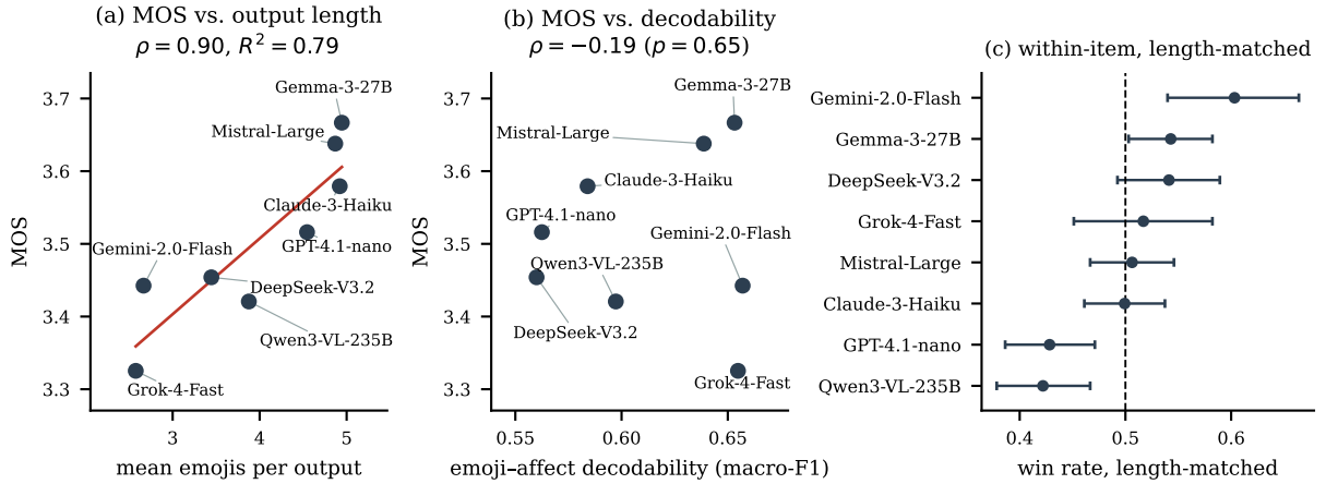
Figure 2: (a) Mean output length explains 78.7% of between-system MOS variance. (b) Emoji-affect decodability does not correlate with MOS. (c) Within-item length-matched win rates reorder the leaderboard; error bars are 95% binomial CIs.
