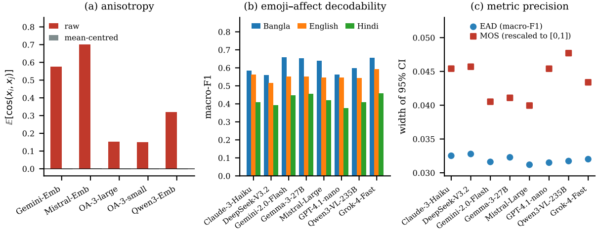
Figure 3: (a) Provider anisotropy differences vanish under mean-centring. (b) Emoji-affect decodability by system and language. (c) Width of the 95% CI for EAD and for MOS rescaled to a common range; EAD is the more precise instrument.
