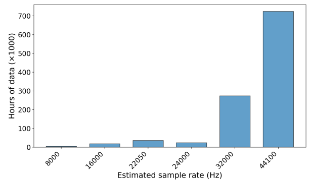
Figure 4: YODAS v3 data distribution by estimated effective bandwidth; over 92% of recordings exceed 32 kHz.
