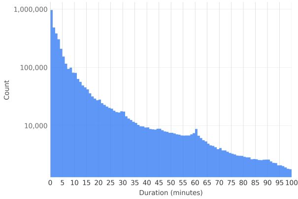
Figure 3: Distribution of videos by total length (log scale), bucketed into groups by minute.
