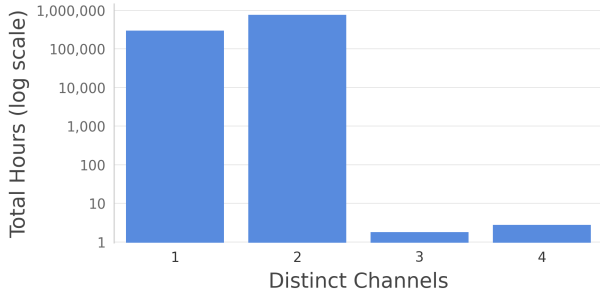
Figure 5: Log-scale distribution of data by effective number of channels in each audio file
