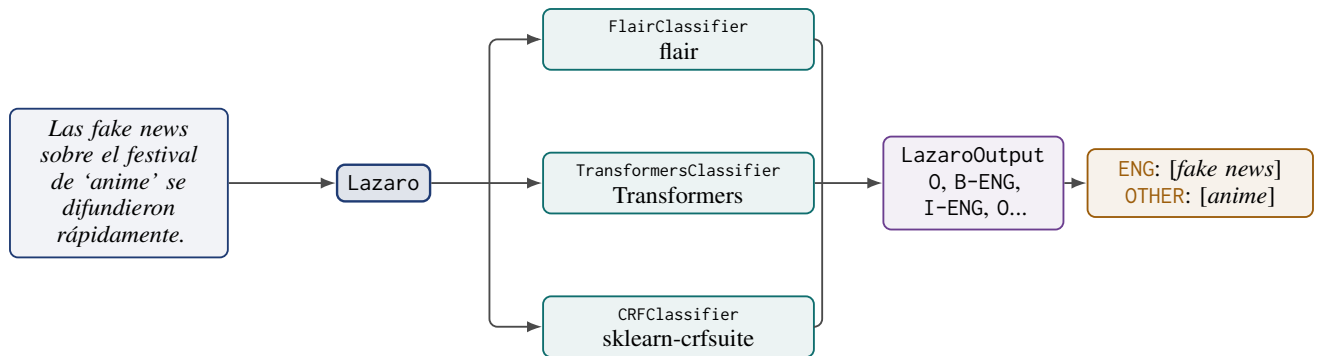
Figure 1: Architecture of pylazaro. The Lazaro class receives the input text and dispatches it to the classifier that corresponds to the model selected by the user. Each classifier loads its model using the library it was trained with and returns a sequence of BIO tags, which are wrapped in a common output object that implements the different output formats. Adding a new model only requires implementing a new classifier.
