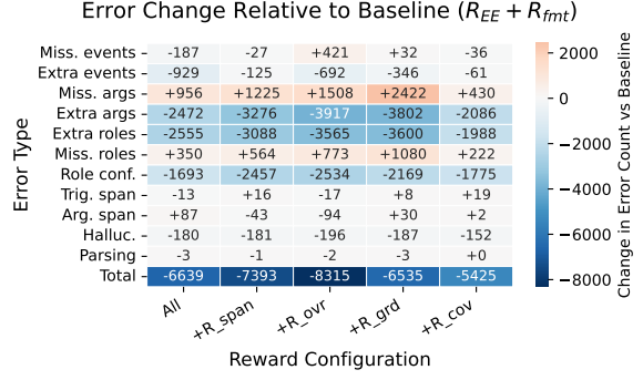
Figure 5: Error Change Relative to Baseline ( R_{EE} + R_{fmt} ).
