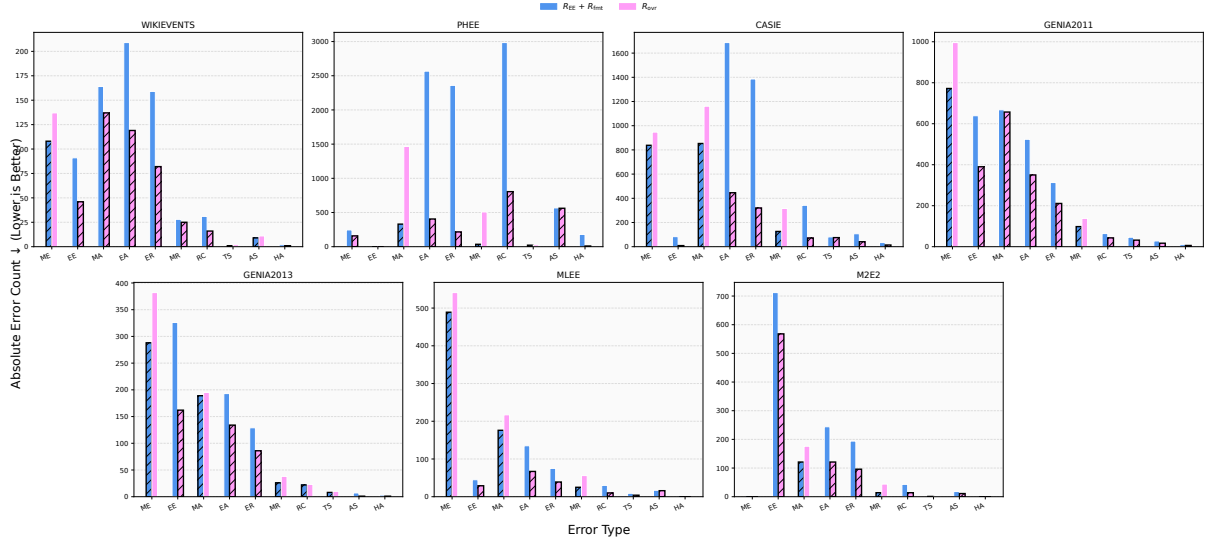
Figure 10: Comparative evaluation of error categories across datasets. R_{EE} + R_{fmt} Vs. +R_{ovr}
