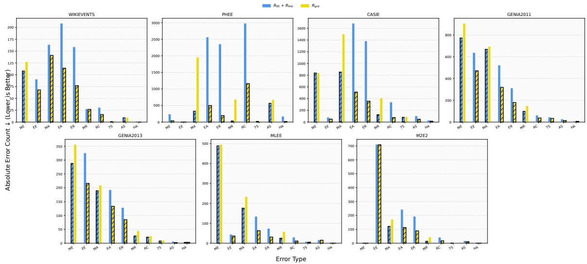
Figure 11: Comparative evaluation of error categories across datasets. R_{EE} + R_{fmt} Vs. +R_{grd}
