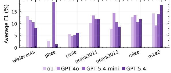
Figure 1: Average-F1 performance of frontier LLMs on end-to-end event extraction across 7 datasets and domains.
