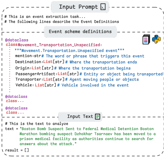
Figure 2: Structure of a prompt for end-to-end Event Extraction, comprising a task instruction a set of event schemas and the input text.
