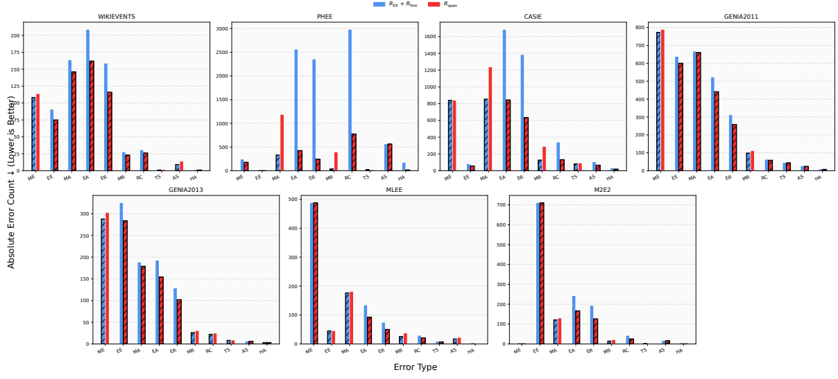
Figure 9: Comparative evaluation of error categories across datasets. R_{EE} + R_{fmt} Vs. +R_{span}
