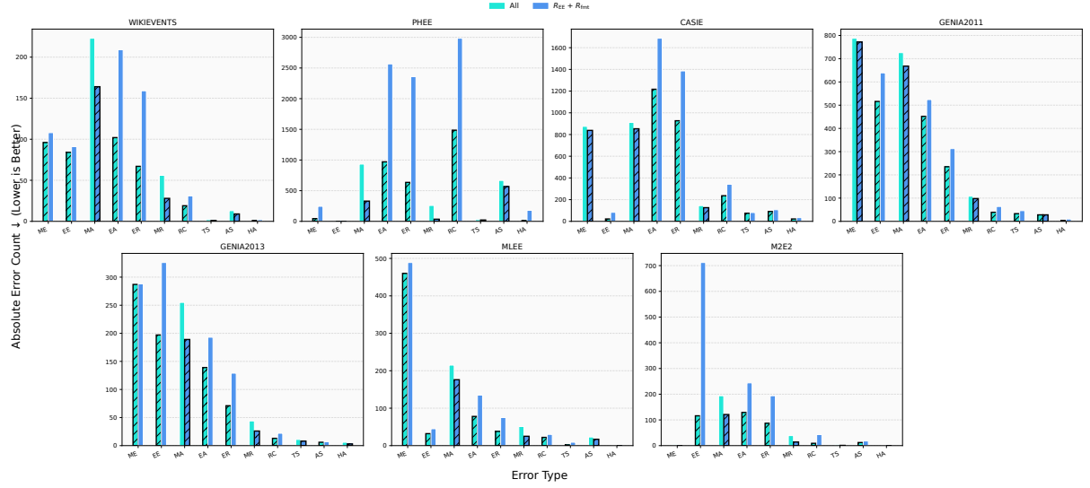
Figure 13: Comparative evaluation of error categories across datasets. R_{EE} + R_{fmt} Vs. All
