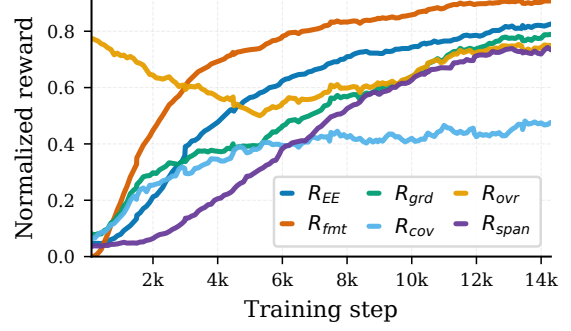
Figure 4: Training rewards dynamics.
