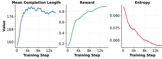
Figure 8: Analysis of the main metrics for monitoring our RL training dynamics including the mean completion length, the mean reward score, and generation entropy.
