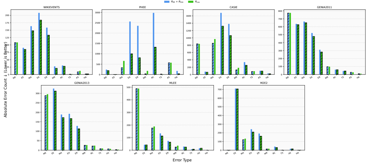
Figure 12: Comparative evaluation of error categories across datasets. R_{EE} + R_{fmt} Vs. +R_{cov}
