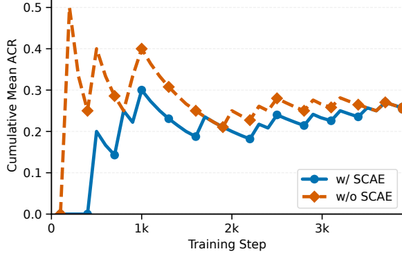
Figure 3: Cumulative Mean ACR during training
