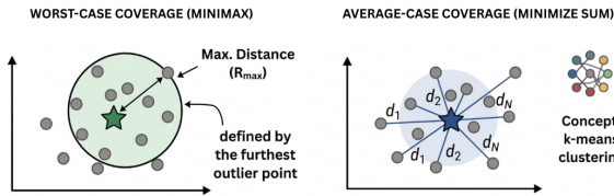
Fig. 2. Prototype-selection objectives: minimax (left) and average-case (right).
