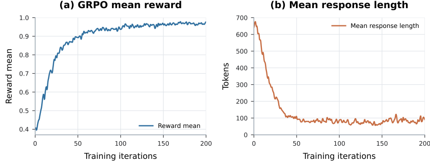
Figure 2: GRPO mean rewards (left) and mean response length in tokens (right) by training steps.
