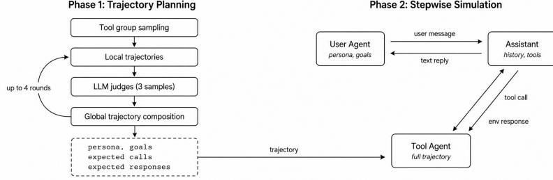
Figure 3: Dialogue generation pipeline. A planner constructs a structured trajectory from a sampled tool group and refines it through up to four rounds of judge feedback. The trajectory is then handed to a three-agent stepwise simulation in which the User Agent, Assistant, and Tool Agent operate under asymmetric visibility; flagged erroneous assistant turns remain in context but are never used as training targets.
