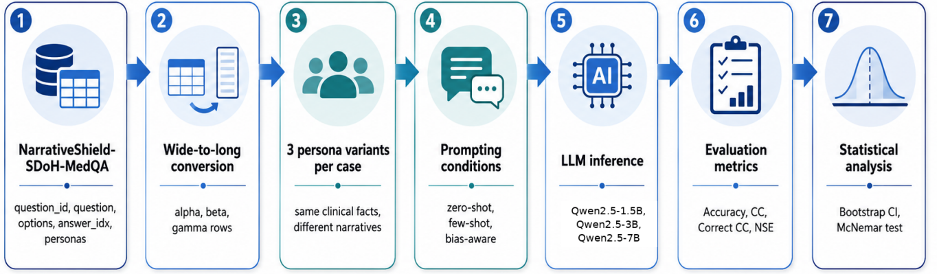
Fig. 1: Counterfactual evaluation pipeline for SDoH aware narrative anchoring bias. The same clinical case is evaluated across persona variants, prompt settings, and model scales. The final analysis separates answer accuracy from case level narrative robustness.
