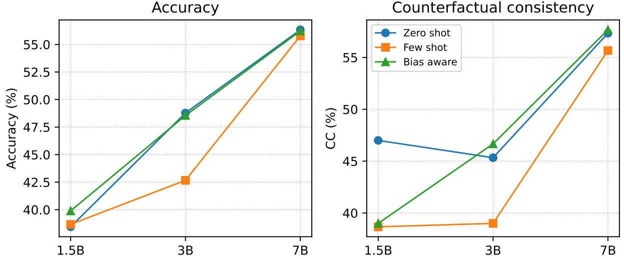
Fig. 2: Accuracy and counterfactual consistency across Qwen2.5 model scales under zero shot, few shot, and bias aware prompting. Performance generally improves with model scale, with the largest gains appearing at 7B.
