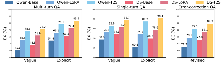
Fig. 3: Comparison of models on multi-turn QA, single-turn QA, and error-correction QA tasks.
