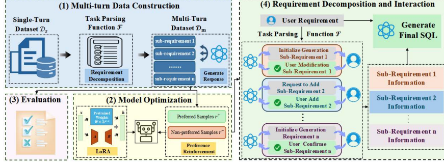
Fig. 1: The workflow of SPOC-SQL. (1) The task parsing function \mathcal{F} decomposes single-turn queries into multi-turn sequences with stage-specific sub-requirements. (2) LoRA fine-tuning combined with preference-based optimization to enhance decision capability through fine-grained policy optimization. (3) Evaluation of multi-turn QA capabilities. (4) At inference, \mathcal{F} decomposes user requirements into sub-tasks for iterative confirmation, generating the final SQL.
