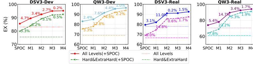
Fig. 2: Performance of SPOC-SQL across different datasets and models: Evaluations on DeepSeekV3(DSV3) and Qwen3-72B(QW3) across Spider-Dev(Dev) and Spider-Realistic(Real) Datasets.
