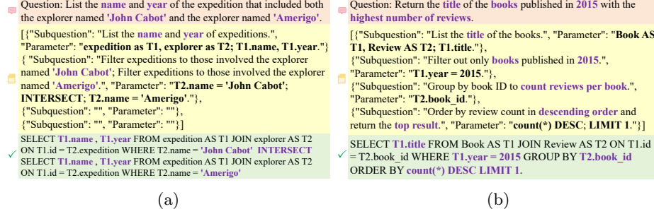
Fig. 4: Case Study: (a) Decomposition of complex nested queries and set operations; (b) Modular parsing of multi-component SQL queries.
