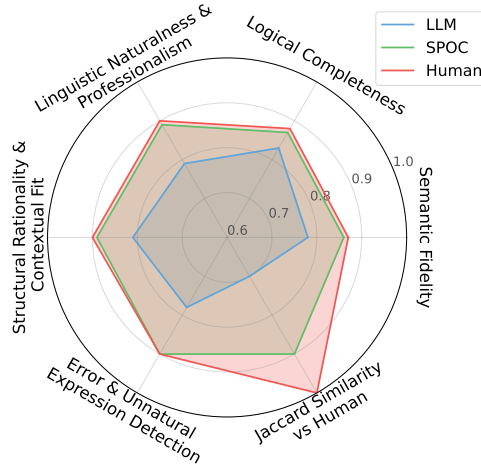
Fig. 5: Comparison of SQL Info versions across subjective and objective metrics.
