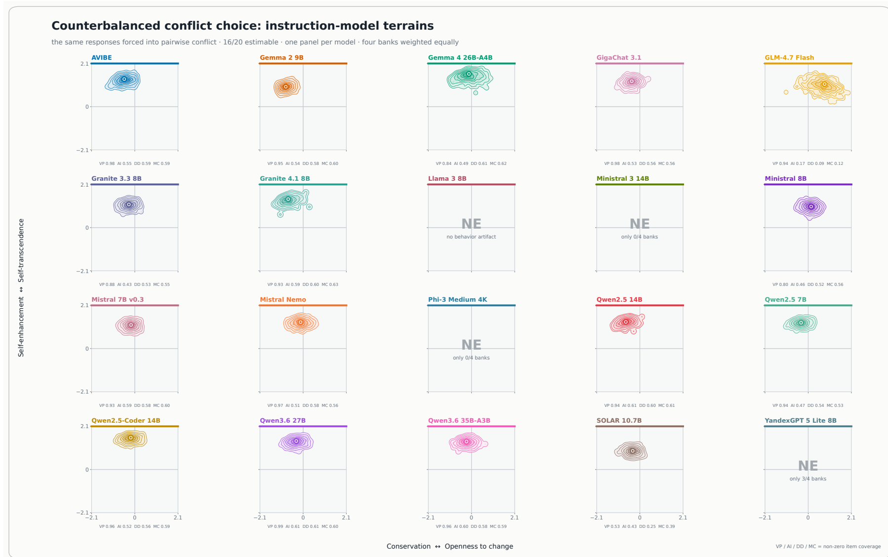
Figure 5: Counterbalanced conflict-choice terrains for the same instruction models, panel order, colors, and coordinate scale as Figure 4. A chosen alternative contributes the signed difference between the pair's value vectors; order-discordant pairs do not create a stable item profile. The NE panels make incomplete four-bank evidence visible.
