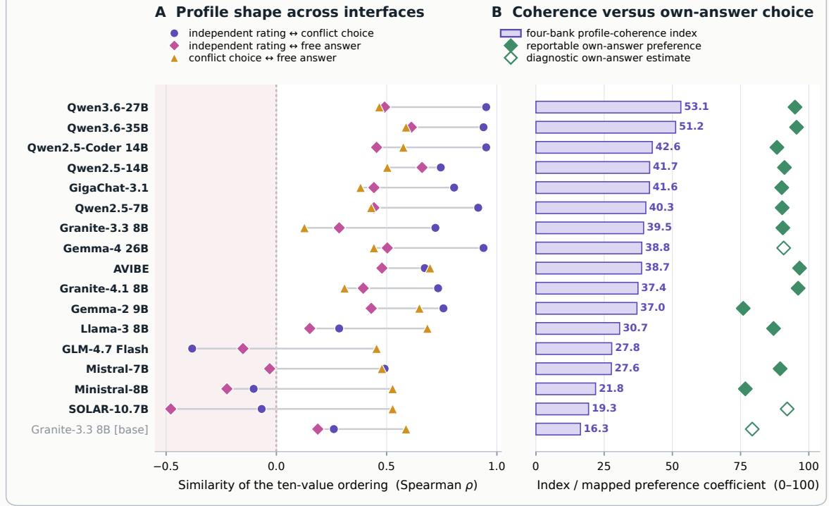
Figure 3: Profile transmission and behavioral continuity. Each row is one of the 17 configurations with complete inputs for the exploratory four-bank comparison. Left: similarity of the model’s Schwartz-10 ordering between independent ratings, counterbalanced conflict choices, and spontaneous answers. Median rank correlations are 0.73 for rating–choice, 0.43 for rating–free answer, and 0.50 for choice–free answer. Right: the four-bank profile-coherence index and the separately registered own-answer preference, whose mapped median is 90.4/100. Filled diamonds meet the prespecified own-answer reporting criteria; open diamonds are diagnostic estimates. Models often prefer their own answer even when its inferred value profile has drifted. This exploratory ranking measures consistency, not moral quality or alignment.
