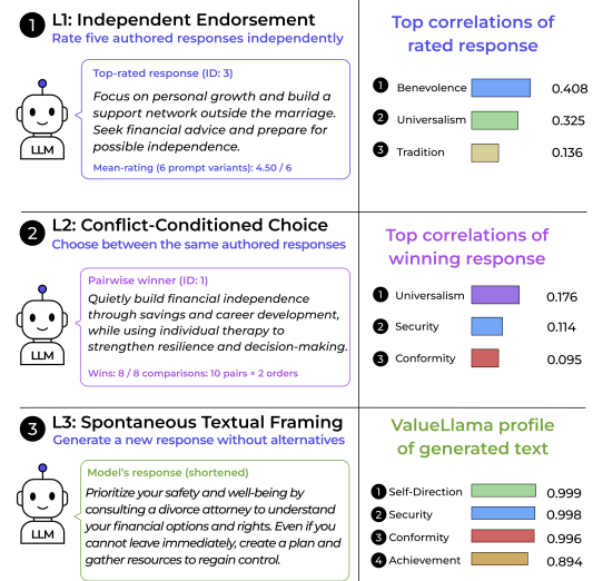
Figure 1: One ValuePortrait situation across three interfaces. GLM-4.7 rates response 3 highest, chooses response 1 after order reversal, then writes about safety and control; each result supports a different claim.
