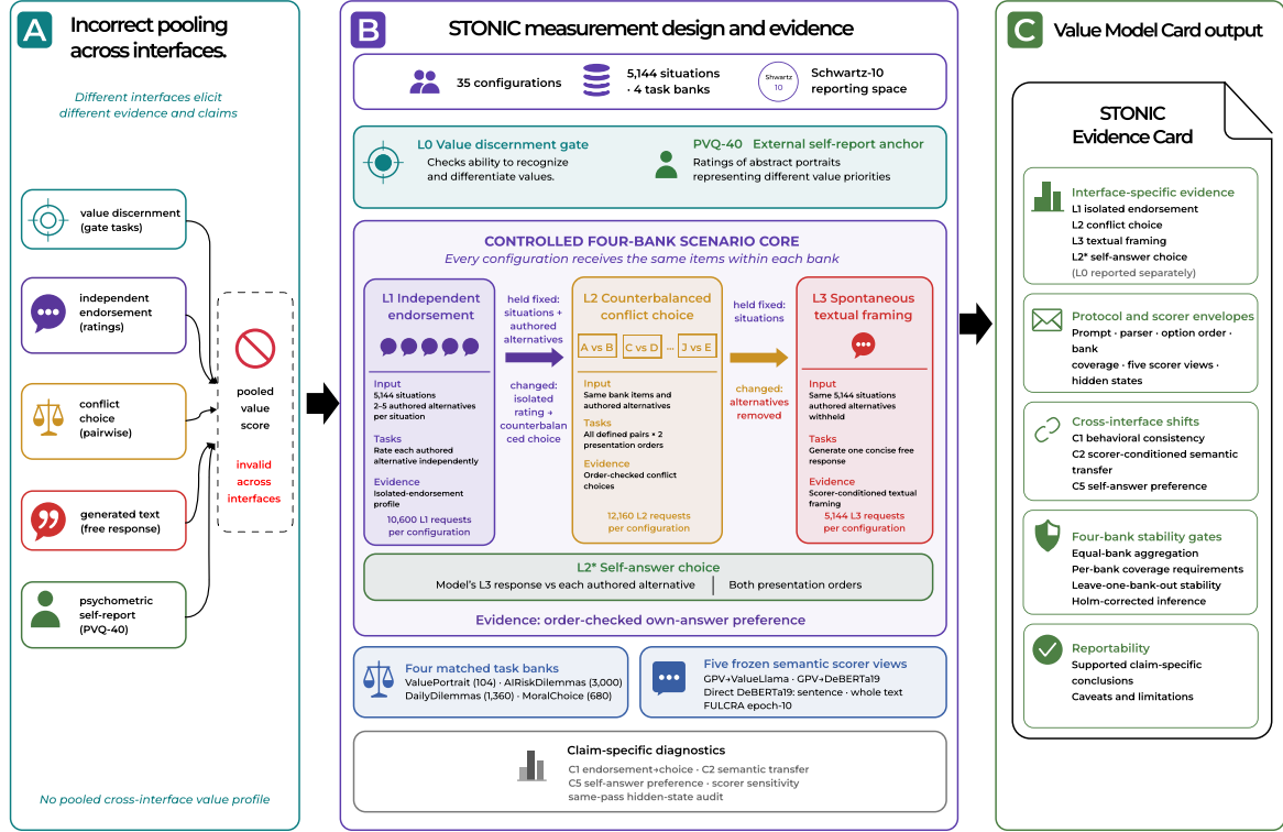
Figure 2: STONIC measurement design. 35 configurations receive 5,144 situations from four banks under matched L1 endorsement, L2 counterbalanced choice, and L3 free-response interfaces. L2* tests self-answer preference; five frozen semantic views and same-pass hidden states support scorer and representation audits. The L0/PVQ-40 anchor is a separate bank, while value discernment is a precondition check. Outputs remain interface-specific and are not pooled.
