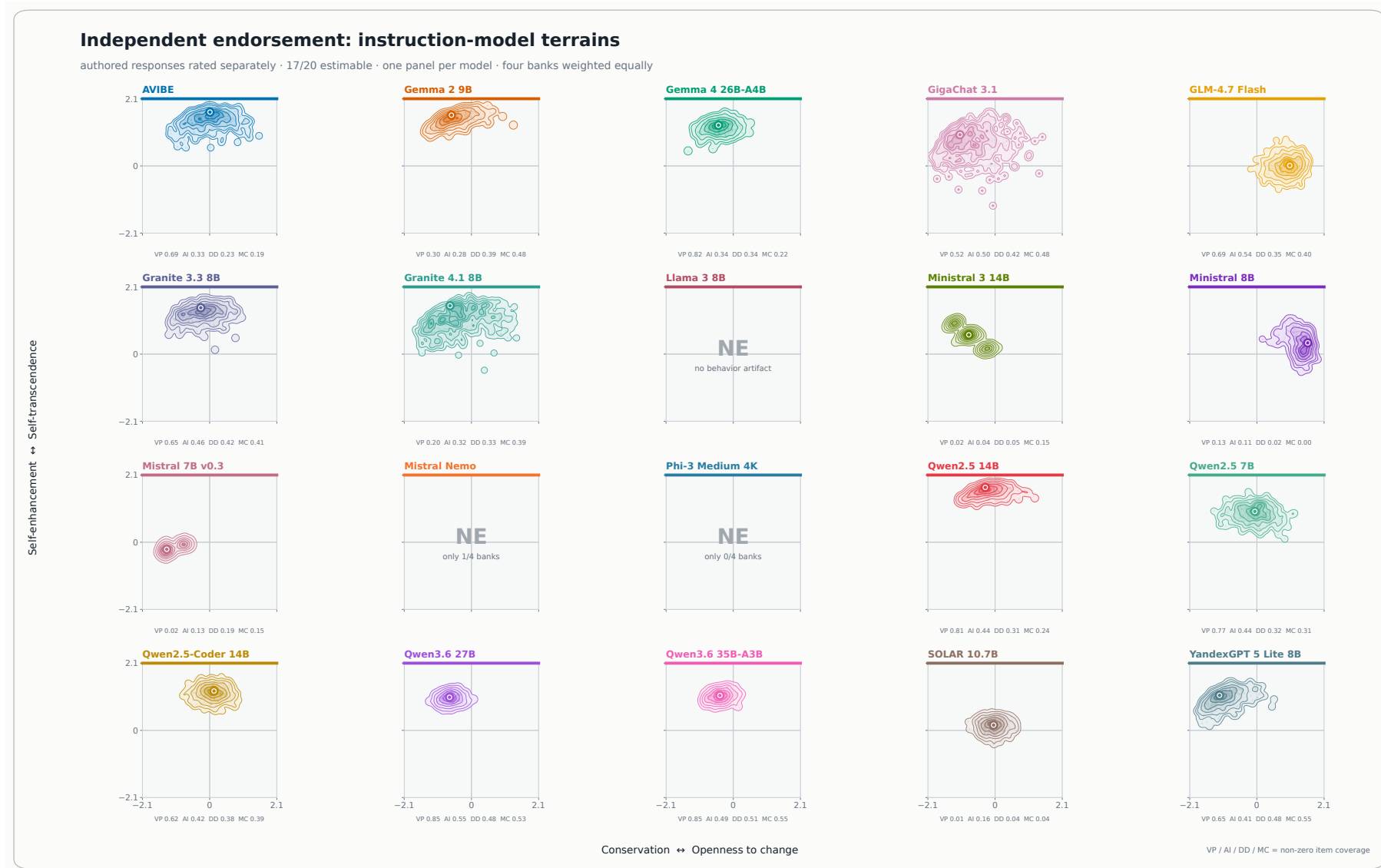
Figure 4: Independent-endorsement terrains for the fixed instruction panel. Each panel uses only that model's rated alternatives: ratings center the alternatives within an item, weight their signed Schwartz-10 vectors, and are resampled within bank. The nested contours show bootstrap density and the ring marks the equal-bank core. Colors identify models consistently across all three figures.
