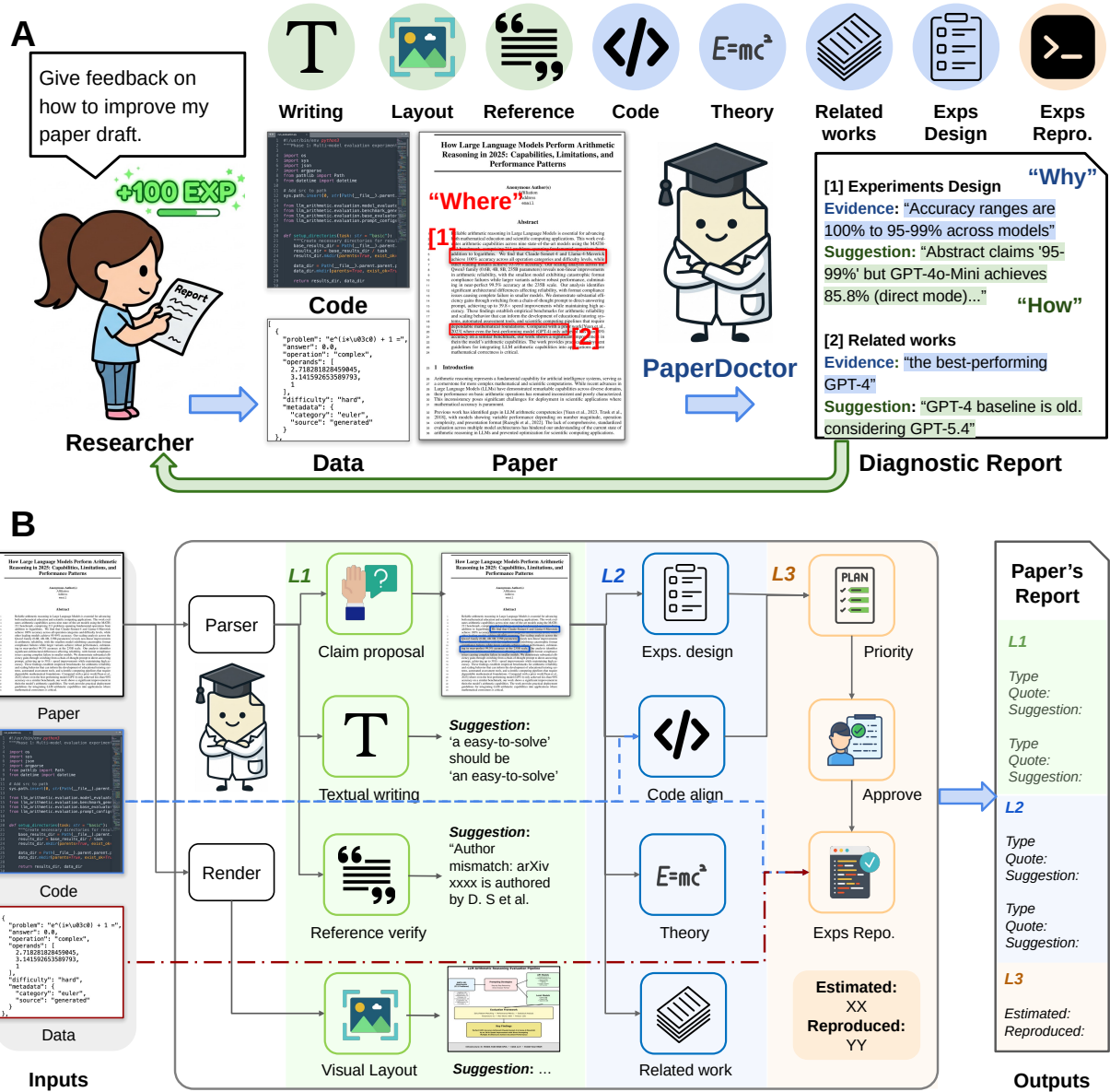
Figure 1: A. PaperDoctor agent provides evidence-grounded, actionable feedback. Given a paper along with its code and datasets, PaperDoctor returns a holistic report of findings across multiple dimensions (writing, citations, figures, equations, code, reproduction, and related work). Each finding pairs an error type ( Why ) with a concrete suggestion ( How ) and is grounded ( Where ) in the paper itself, allowing authors to audit and learn from every critique. B. Illustration of PaperDoctor pipeline. PaperDoctor runs three diagnostic stages: L1 paper-only screening (Sec. 2.2), L2 typed claim verifiers (Sec. 2.3), and L3 prioritised experiment reproduction (Sec. 2.4), to produce evidence-grounded, actionable feedback on pre-submission papers.
