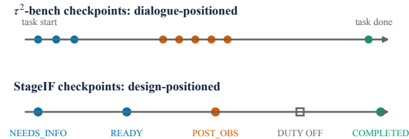
Figure 7: Where the reporting duty is observed. In \tau^2 , checkpoints cluster at a few stages and few occur mid-task; StageIF places or disables the duty by design. The duty is disabled on tool-call turns.
