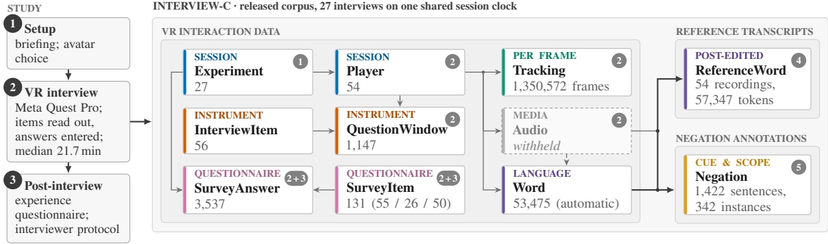
Figure 1: Study flow (left: the three stages of each session) and the InterView-C corpus (right), whose three released parts share one session clock. VR interaction data : records per table (fingers tracked in 515,995 / 544,280 frames; SurveyItem: 55 interview, 26 protocol and 50 experience items); thin arrows are record links, the dashed arrow marks automatic transcription and thick arrows mark derivation. The reference transcripts are post-edited from the automatic transcript against the withheld audio and the negation annotations are sampled from it. Badges give the creating stage; 4 (post-editing) and 5 (annotation) continue the study stages.
