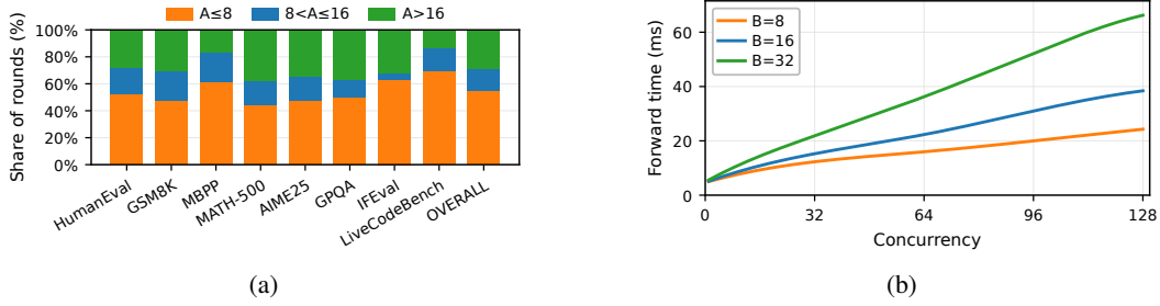
Figure 2: Acceptance variability and block-dependent forward cost of self-speculation. (a) Acceptance length distribution with B = 32 . (b) Forward time across concurrency levels for B \in \{8, 16, 32\} .
