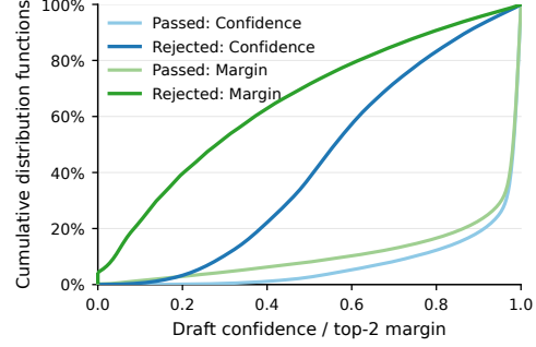
Figure 3: Cumulative distribution functions (CDFs) of draft confidence and top-2 probability margin during drafting rounds.
