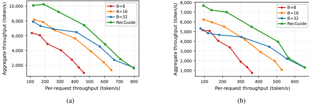
Figure 5: Aggregate and per-request throughput trade-offs under different concurrency levels on (a) NLD-8B and (b) NLD-14B. We compare fixed block sizes B \in \{8, 16, 32\} with RecGuide.
