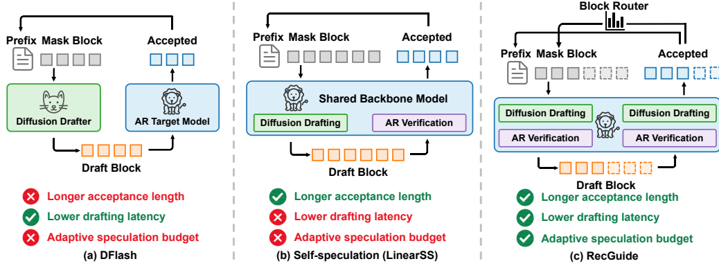
Figure 1: Comparison between RecGuide and existing diffusion-based speculative decoding.
