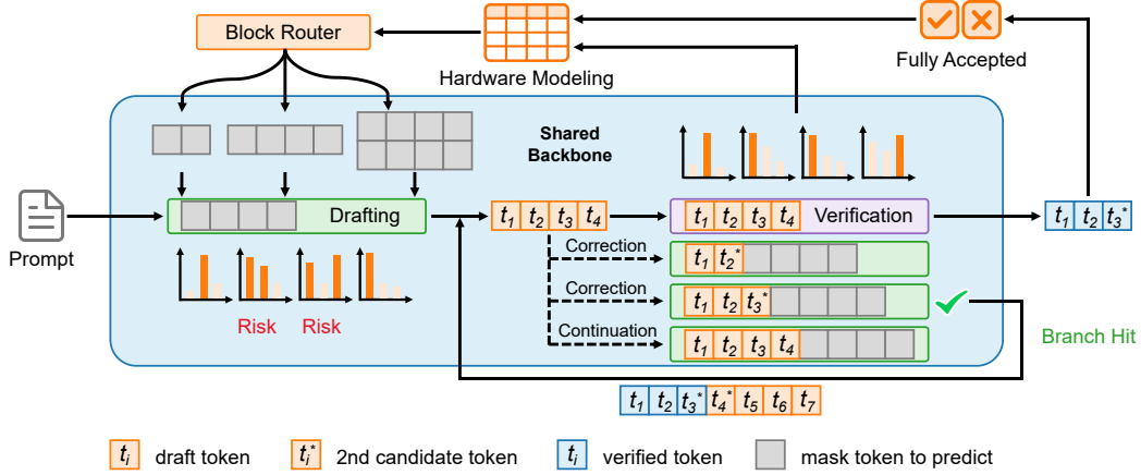
Figure 4: Overview of RecGuide runtime orchestration. Draft uncertainty guides predictive draft-verify overlap through correction and continuation branches, while verification feedback and hardware profiles guide request-specific block size allocation.
