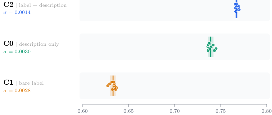
Figure 1 10 random permutations of option order across three variants on MMLU. Standard deviation is measured.
