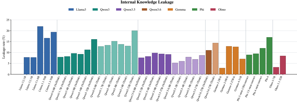
Figure 3: Internal knowledge leakage across models. Leakage measures the extent to which models produce answers by relying on internal parametric knowledge rather than the provided context. Colors indicate different model families, and model sizes increase from left to right within each family.
