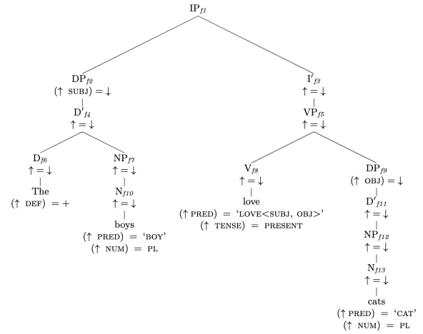
Figure 4: C-structure. Labels (e.g., f_1 , f_2 ) are provided in the c-structure, where f_1 refers to the f-structure associated with the IP node and so on.
