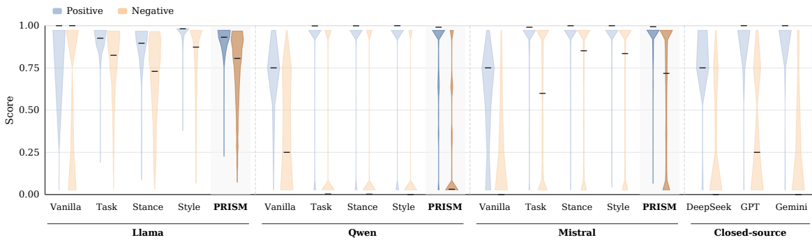
Figure 14: Score distribution on the Big5-Persona-EASY dataset
